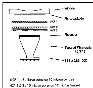
Figure 12: UVOT detector.
