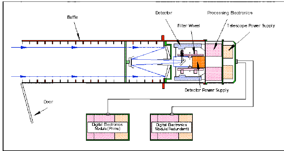
Figure 10: UVOT Schematic.
