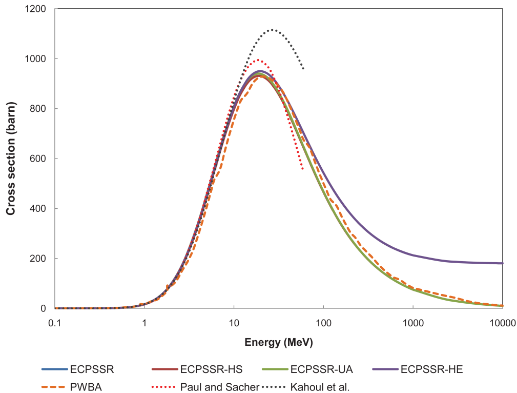
Fig. 10.1: Cross section for the ionisation of copper K shell by proton impact according to the various implemented modeling options: ECPSSR model, ECPSSR model with “united atom” (UA) approximation, Hartree-Slater (HS) corrections and specialized for high energies (HE); plane wave Born approximation (PWBA); empirical models by Paul and Sacher and Kahoul et al. The curves reproducing some of the model implementations can be hardly distinguished in the plot due to their similarity.
