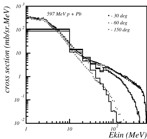
Fig. 26.11: Double differential cross-section for neutrons produced in proton scattering off Lead. Proton incident energy was 597 MeV. The points are data, the histogram is Binary Cascade prediction.
