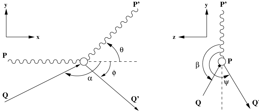
Fig. 7.1: Scattering diagram of atomic bound electron Compton scattering. \mathbf{P} is the incident photon momentum, \mathbf{Q} the electron pre-collision momentum, \mathbf{P}' the scattered photon momentum and \mathbf{Q}' the recoil electron momentum.
