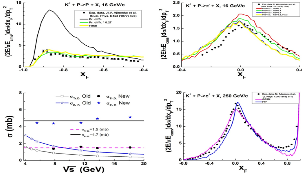
Fig. 24.13: Upper figures: inclusive spectra of protons and \pi^+ -mesons in K^+ p -interactions. Points are experimental data [had-Ajinenko,had-Ajinenko2]. Lines are FTF calculations. Bottom left figure: diffraction dissociation cross sections obtained by tuning (points), and their description (lines) by the expression for Kp in (24.4). Bottom right figure: x_F spectrum of positive charged particles in Kp -interactions at p_{\text{lab}} = 250 GeV/c. Points are experimental data [Whi74], lines are model calculations.
