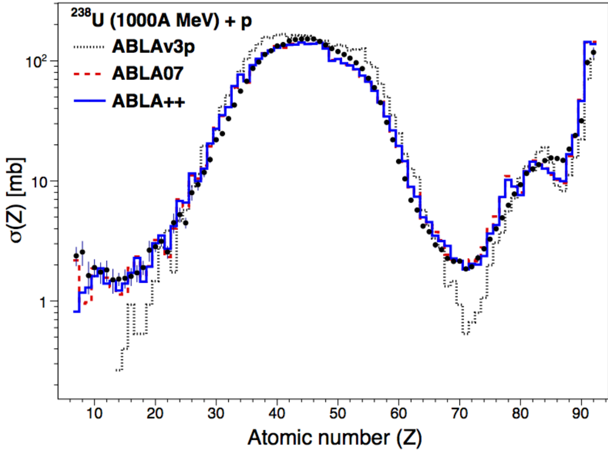
Fig. 33.1: ABLA calculations performed with the fortran version (ABLA07), the new one in C++ (ABLA++) and the previous version (ABLA3p) are compared with the atomic-number distribution of fission and evaporation residues produced in the reactions p + {}^{238}\text{U} at 1A GeV.
