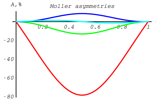
Fig. 14.6: Differential cross section asymmetries in % for Møller scattering (red - A_{ZZ}(\epsilon) , green - A_{XX}(\epsilon) , blue - A_{YY}(\epsilon) , light blue - A_{ZX}(\epsilon) )
