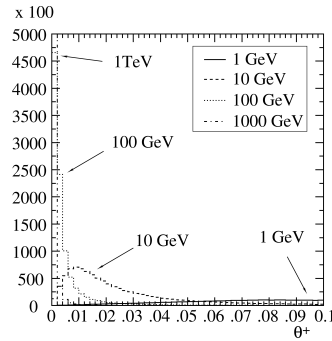
Fig. 7.12: Histograms of generated \theta_+ distributions at different photon energies.
