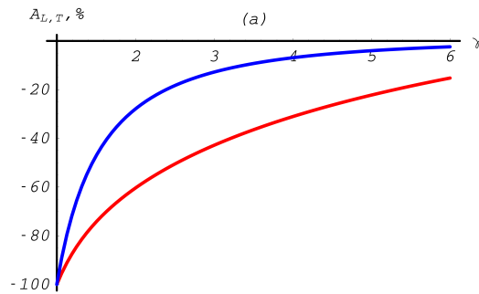
Fig. 14.12: Annihilation total cross section asymmetries depending on the total energy of the incoming positron E_{k_1} . The transverse asymmetry is shown in blue, the longitudinal asymmetry in red.
