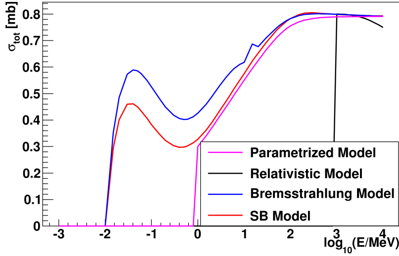
Fig. 11.1: Total cross section comparison between models for Z = 29 : Parametrized Bremsstrahlung Model, Relativistic Model, Bremsstrahlung Model (GEANT4 9.4) and Seltzer-Berger Model. The discontinuities in the Parametrized Model and the Relativistic Model at 1 MeV and 1 GeV, respectively, mark the validity range of these models.
