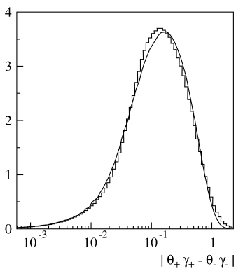
Fig. 7.15: Distribution of the difference of transverse momenta of positive and negative muons (with logarithmic x-scale).
