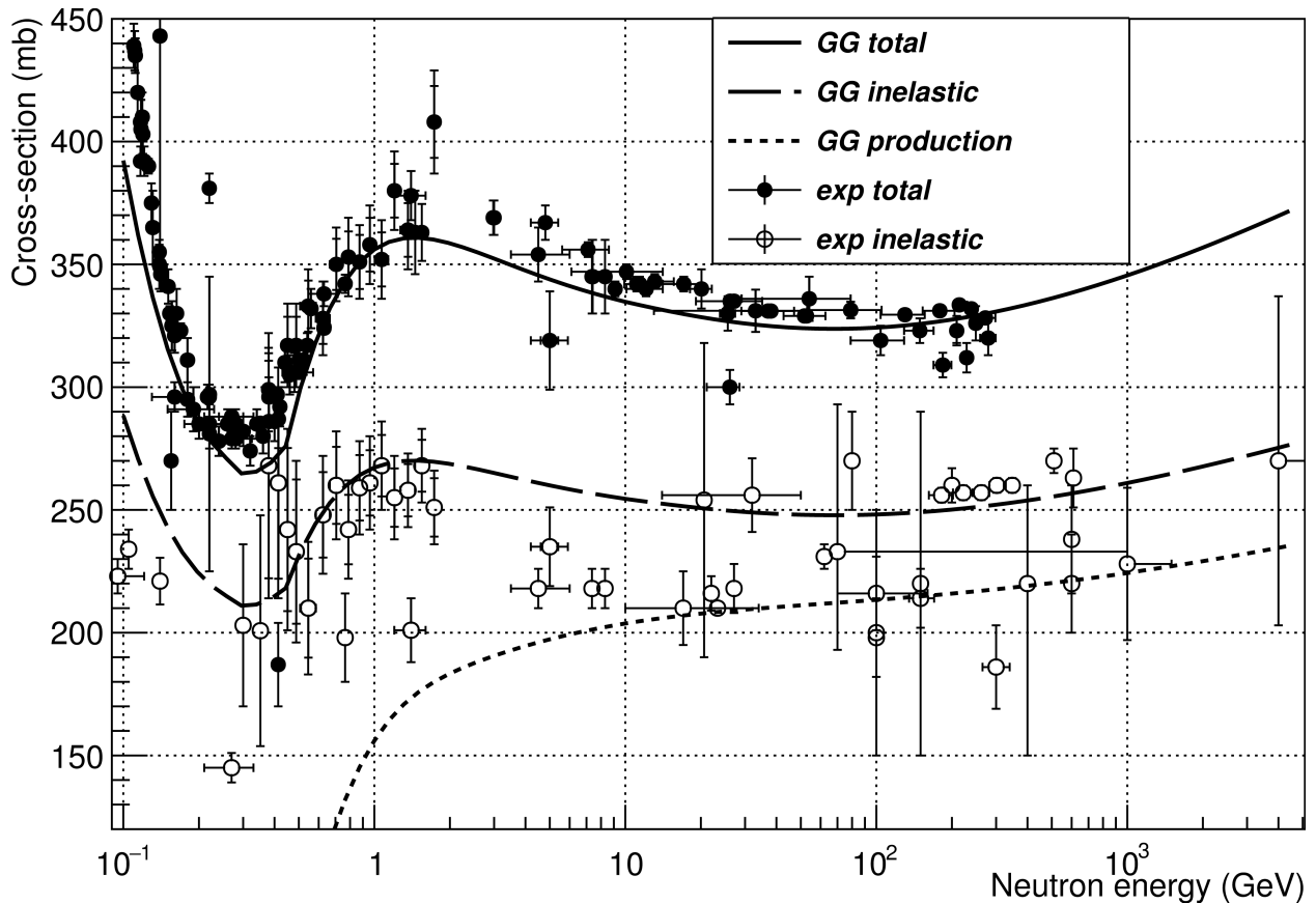
Fig. 20.1: Total, inelastic and production cross-sections of neutrons on a carbon target in the energy range 10^{-2} - 10^3 GeV. Experimental data (open and solid points) from [IHEP, NEA], lines correspond to the Glauber-Gribov model.
