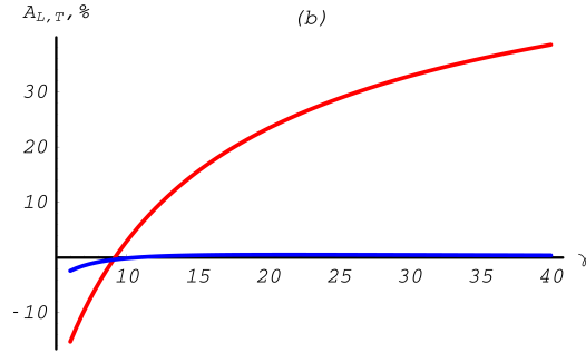
Fig. 14.13: Annihilation total cross section asymmetries depending on the total energy of the incoming positron E_{k_1} . The transverse asymmetry is shown in blue, the longitudinal asymmetry in red.
