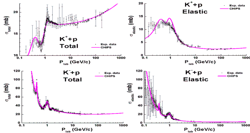
Fig. 24.7: Total and elastic cross sections of Kp -interactions. Points are experimental data from PDG data-base .
