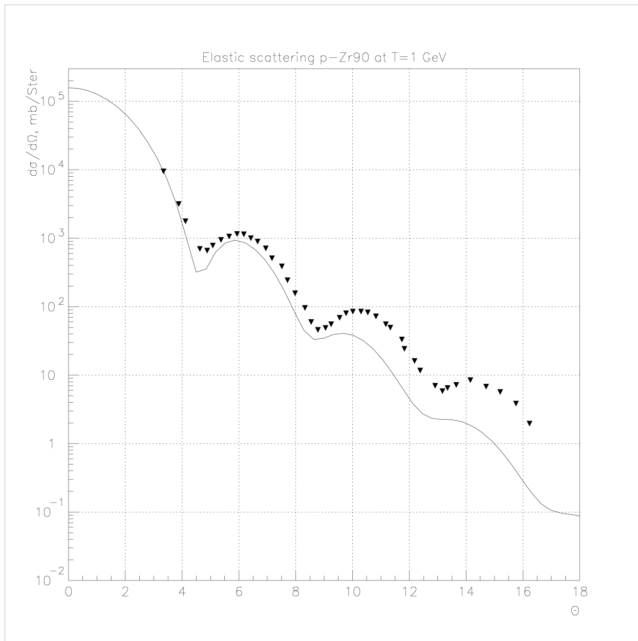
Fig. 22.8: Elastic proton scattering on ^{90}\text{Zr} at 1 GeV.
