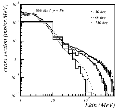
Fig. 26.12: Double differential cross-section for neutrons produced in proton scattering off Lead. Proton incident energy was 800 MeV. The points are data, the histogram is Binary Cascade prediction.
