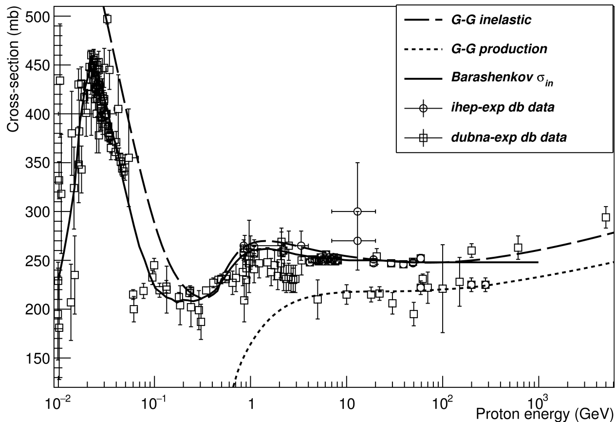
Fig. 20.2: Inelastic and production cross-sections of protons on a carbon target in the energy range 10^{-2} - 10^3 GeV. Experimental data (open points and squares) are from [IHEP, NEA]. The solid and dashed lines correspond to the Barashnikov and Glauber-Gribov inelastic models, respectively. The dotted line shows the Glauber-Gribov production model.
