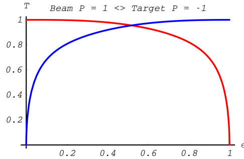
Fig. 14.11: Polarization Transfer in Bhabha scattering. Longitudinal polarization \xi_3^{(2)} of electron with energy E_{p_2} in blue; longitudinal polarization \xi_3^{(1)} of scattered positron. Kinetic energy of incoming positron T_{k_1} = 10\text{MeV}
