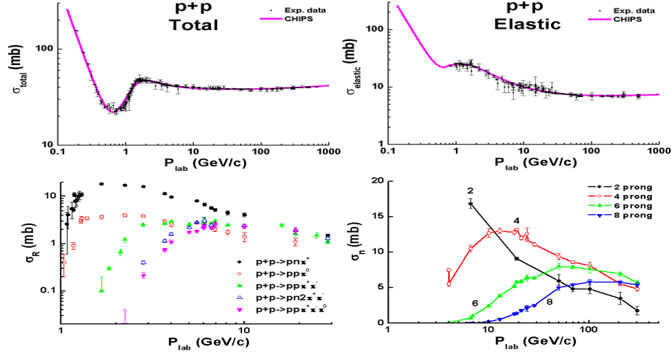
Fig. 24.6: General properties of pp -interactions. Points are experimental data: data on total and elastic cross sections from PDG data-base [PDG12], other data from [eal73a, eal84].
