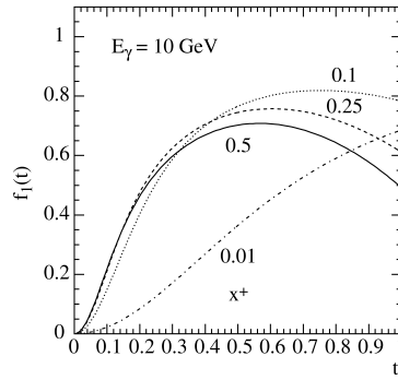
Fig. 7.7: The function f_1(t) at E_\gamma = 10 GeV in beryllium for different values of x_+ .
