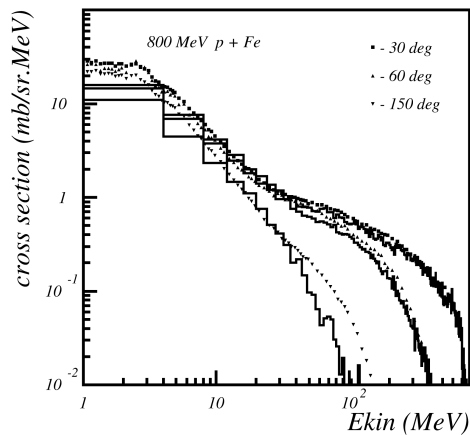
Fig. 26.8: Double differential cross-section for neutrons produced in proton scattering off Iron. Proton incident energy was 800 MeV. The points are data, the histogram is Binary Cascade prediction.
