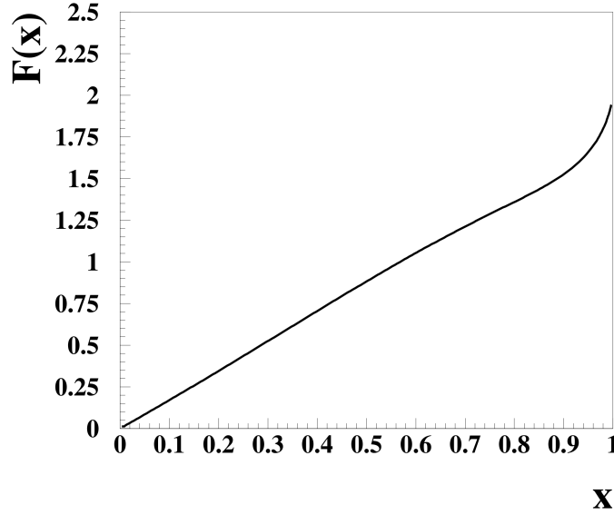
Fig. 5.1: Graph of F(x) ((5.2)).
