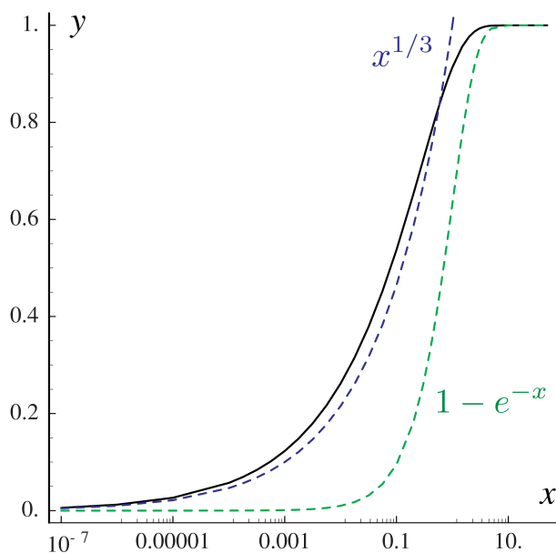
Fig. 15.1: SynFracInt on a log x scale. The functions x^{1/3} , y^3 and 1 - e^{-x} , -\log(1 - y) are shown as dashed lines.
