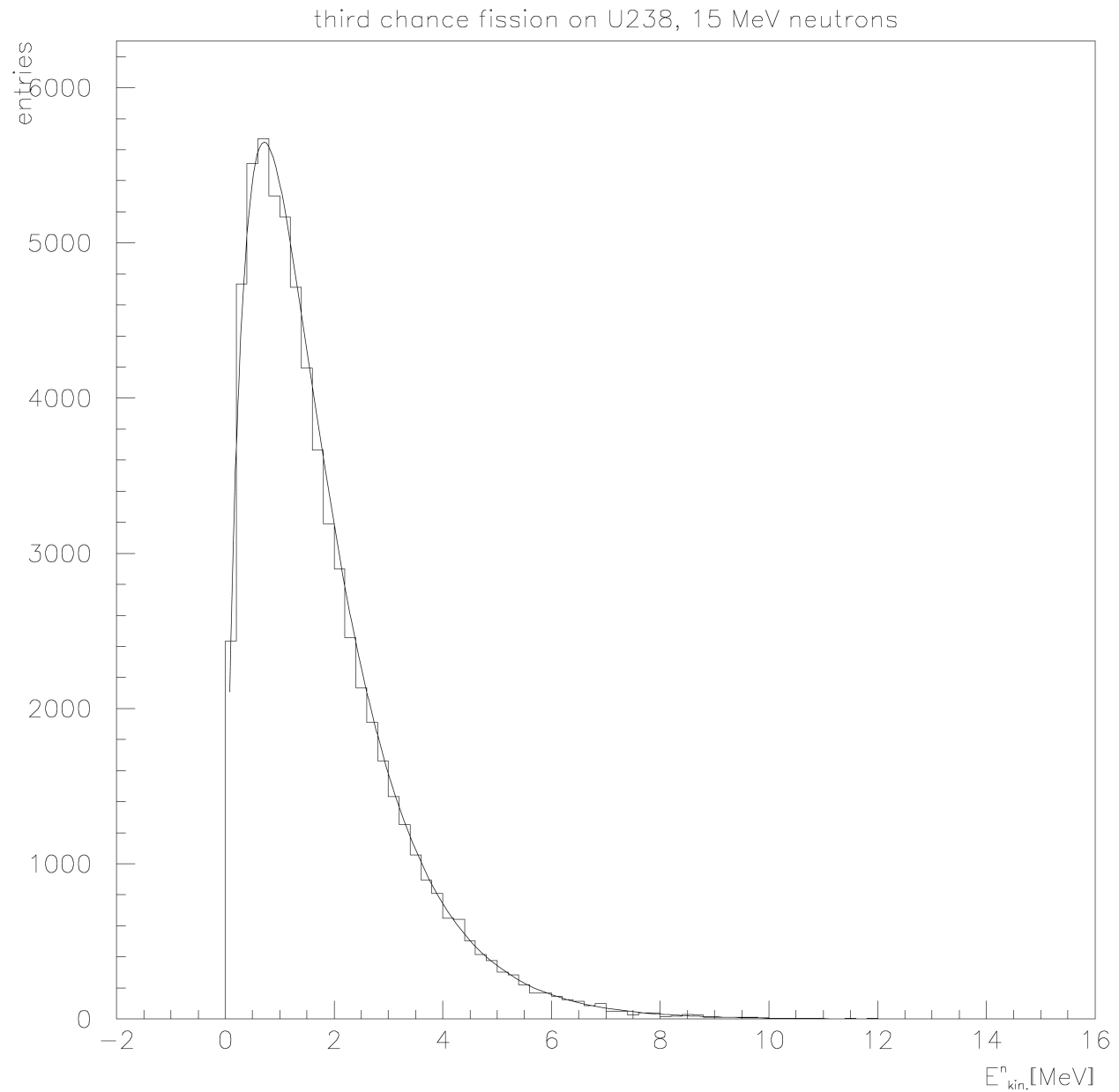
Fig. 38.3: Comparison of data and Monte Carlo for fission neutron energy distributions for induced fission by 15 MeV neutrons on uranium ( ^{238}\text{U} ). The curve represents evaluated data and the histogram is the Monte Carlo prediction.
