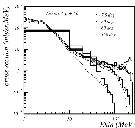
Fig. 26.10: Double differential cross-section for neutrons produced in proton scattering off Lead. Proton incident energy was 256 MeV. The points are data, the histogram is Binary Cascade prediction.
