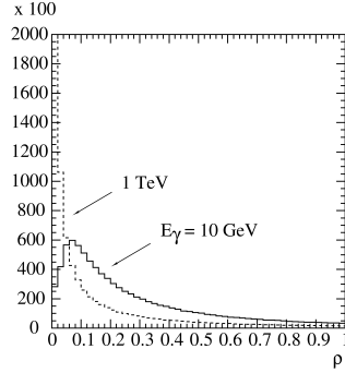
Fig. 7.11: Histograms of generated \rho distributions for beryllium at two different photon energies. The total number of entries at each energy is 10^6 .
