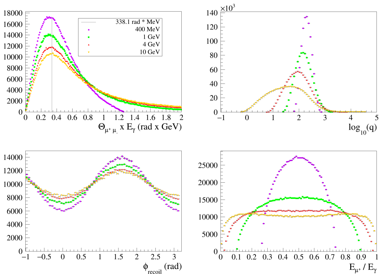
Fig. 7.16: G4BetheHeitler5DModel : \gamma -ray conversions to \mu^+\mu^- pairs on Argon atoms (see text), for various incident-photon energies (bullets 400 MeV, squares 1 GeV, upper triangle 4 GeV, down triangle 10 GeV).
