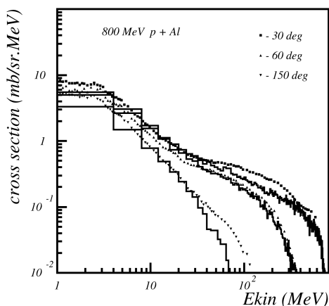
Fig. 26.4: Double differential cross-section for neutrons produced in proton scattering off Aluminum. Proton incident energy was 800 MeV. The points are data, the histogram is Binary Cascade prediction.
