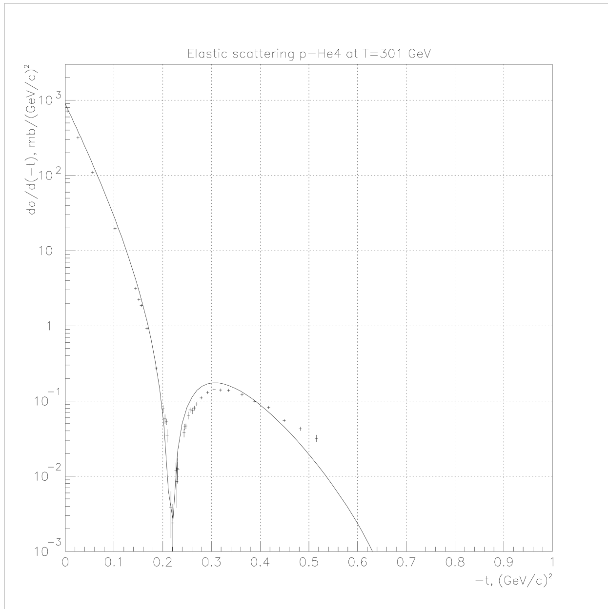
Fig. 22.12: Elastic proton scattering on ^4\text{He} at 301 GeV.
