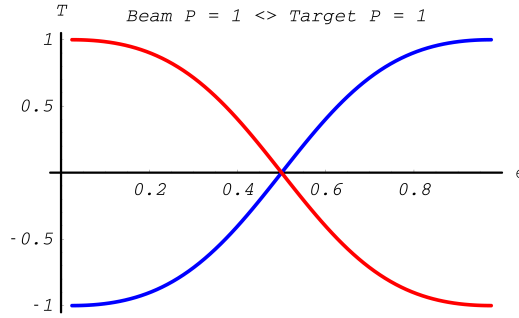
Fig. 14.16: Polarization Transfer in annihilation process. Blue line corresponds to the circular polarization \xi_3^{(1)} of the photon with energy m(\gamma + 1)\epsilon ; red line – circular polarization \xi_3^{(2)} of the photon with energy m(\gamma + 1)(1 - \epsilon) .
