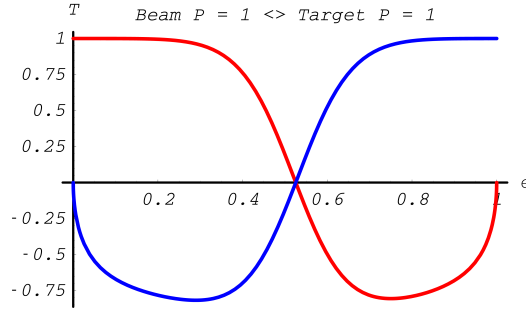
Fig. 14.10: Polarization Transfer in Bhabha scattering. Longitudinal polarization \xi_3^{(2)} of electron with energy E_{p_2} in blue; longitudinal polarization \xi_3^{(1)} of scattered positron. Kinetic energy of incoming positron T_{k_1} = 10\text{MeV}
