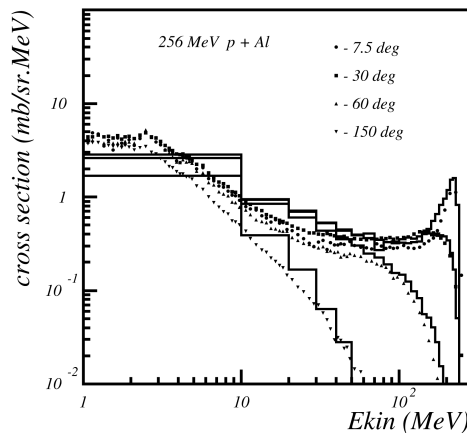
Fig. 26.2: Double differential cross-section for neutrons produced in proton scattering off Aluminum. Proton incident energy was 256 MeV. The points are data, the histogram is Binary Cascade prediction.
