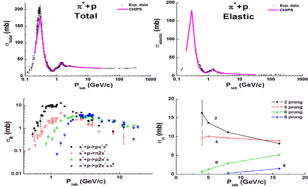
Fig. 24.5: General properties of \pi^+p -interactions. Points are experimental data: data on total and elastic cross sections from PDG data-base [PDG12], other data from [eal72].
