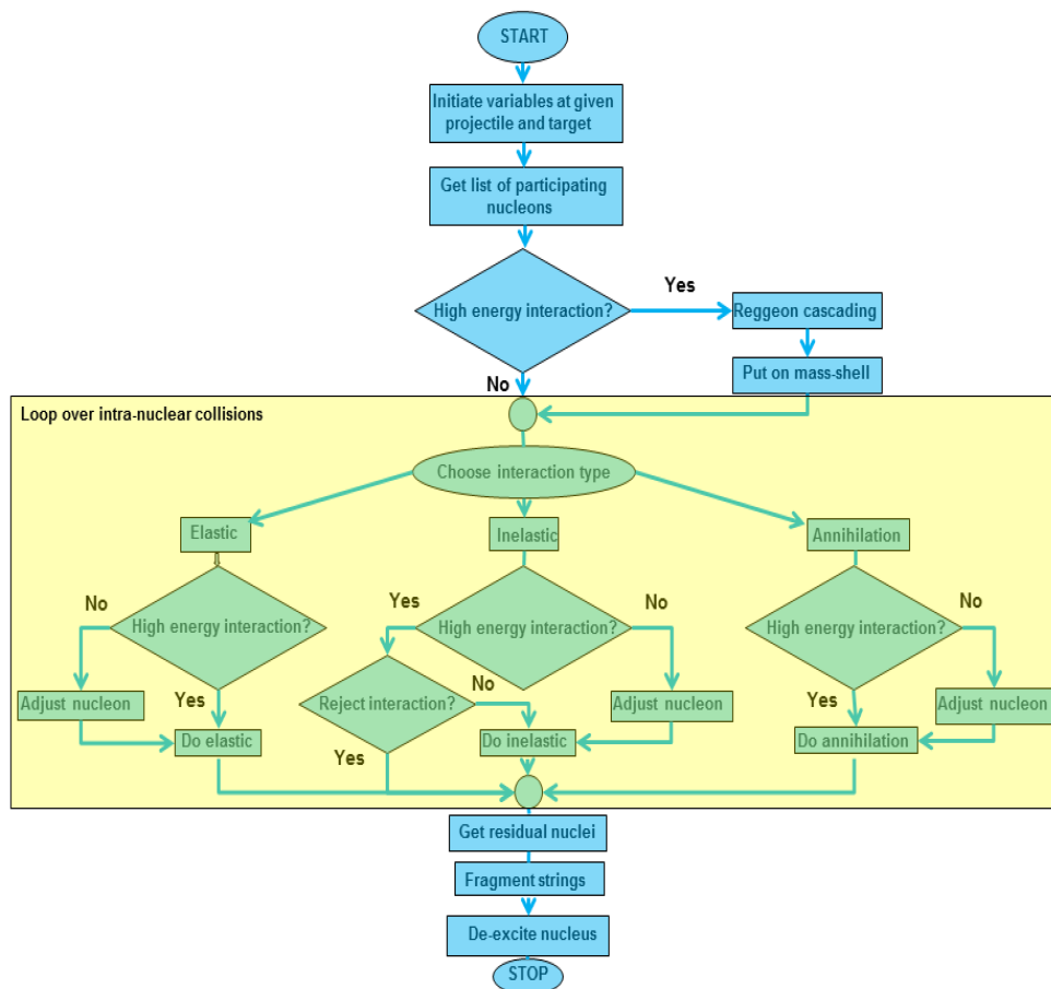
Fig. 24.14: Flowchart of the FTF model.
