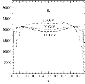
Fig. 7.6: Histogram of generated x_+ distributions for beryllium at three different photon energies. The total number of entries at each energy is 10^6 .
