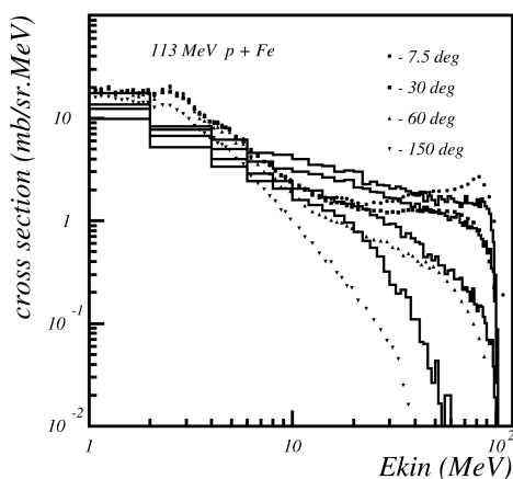
Fig. 26.5: Double differential cross-section for neutrons produced in proton scattering off Iron. Proton incident energy was 113 MeV. The points are data, the histogram is Binary Cascade prediction.
