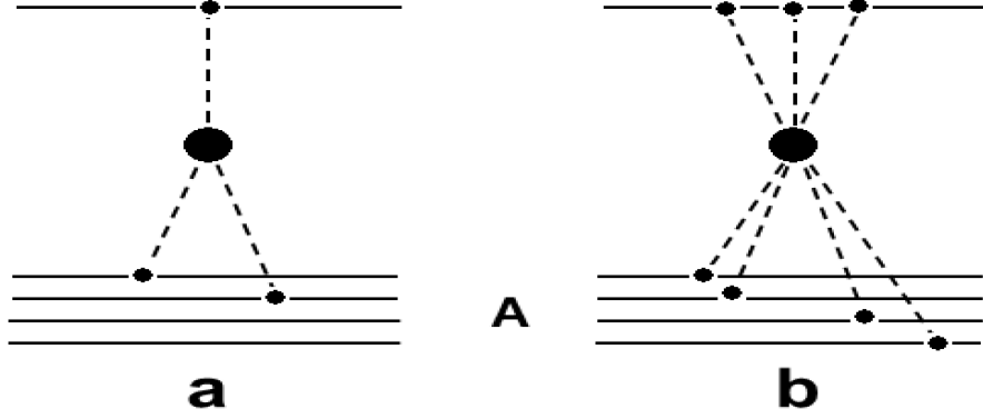
Fig. 24.18: Possible enhanced diagrams of hA -interactions.
