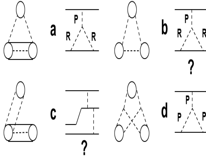
Fig. 24.21: Diagrams of quark-gluon exchanges and corresponding reggeon diagrams for hadron-nucleus interactions.
