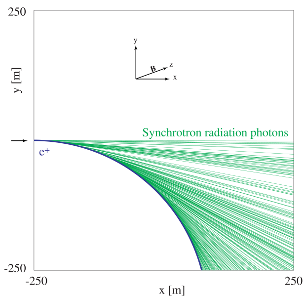
Fig. 15.4: GEANT4 display. 10 \text{ GeV } e^+ moving initially in x-direction, bends downwards on a circular path by a 0.1 \text{ T} magnetic field in z-direction.
