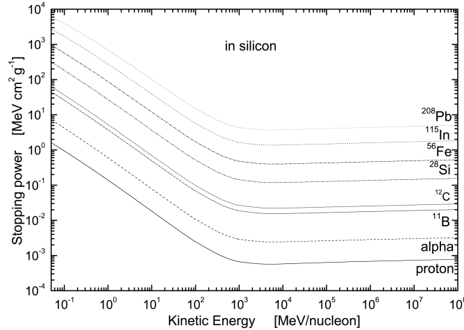
Fig. 9.2: Nuclear stopping power from Ref. [eal11] in \text{MeV cm}^2 \text{g}^{-1} calculated using Eq.(9.30) in silicon shown as a function of the kinetic energy per nucleon from 50 keV/nucleon up 100 TeV/nucleon for protons, \alpha -particles and ^{11}\text{B} , ^{12}\text{C} , ^{28}\text{Si} , ^{56}\text{Fe} , ^{115}\text{In} , ^{208}\text{Pb} nuclei.
