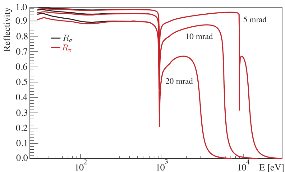
Fig. 7.17: Reflectivity of copper as a function of the photon energy for different impact angles \theta .
