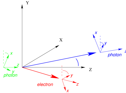
Fig. 14.1: The interaction frame and the particle frames for the example of Compton scattering. The momenta of all participating particle lie in the x - z -plane, the scattering plane. The incoming photon gives the z direction. The outgoing photon is defined as particle 1 and gives the x -direction, perpendicular to the z -axis. The y -axis is then perpendicular to the scattering plane and completes the definition of a right handed coordinate system called interaction frame . The particle frame is defined by the GEANT4 routine G4ThreeMomentum::rotateUz() .
