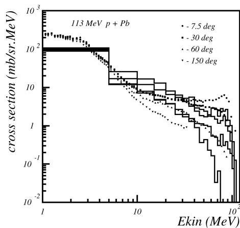
Fig. 26.9: Double differential cross-section for neutrons produced in proton scattering off Lead. Proton incident energy was 113 MeV. The points are data, the histogram is Binary Cascade prediction.
