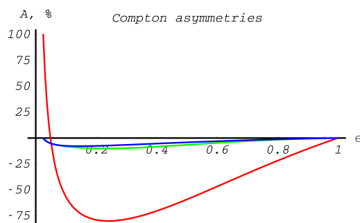
Fig. 14.21: Compton scattering differential cross section asymmetries in%. Red line corresponds to the asymmetry due to circular photon and longitudinal electron initial state polarization, green line – due to circular photon and transverse electron initial state polarization, blue line – due to linear photon and transverse electron initial state polarization.
