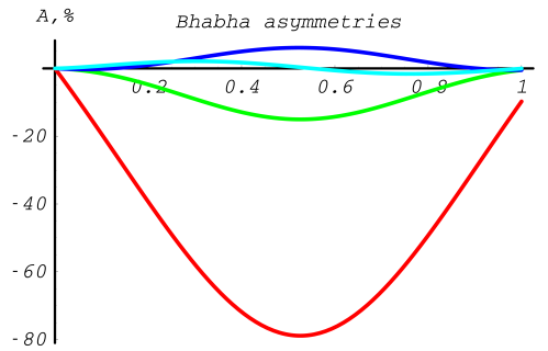
Fig. 14.7: Differential cross section asymmetries in % for Bhabha scattering (red - A_{ZZ}(\epsilon) , green - A_{XX}(\epsilon) , blue - A_{YY}(\epsilon) , light blue - A_{ZX}(\epsilon) )
