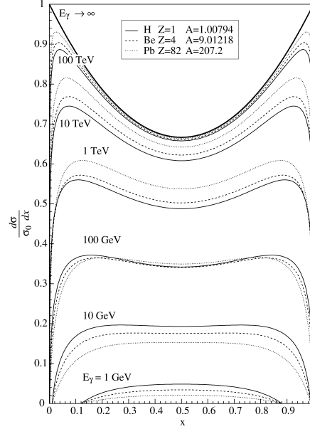
Fig. 7.3: Normalized differential cross section for pair production as a function of x , the energy fraction of the photon energy carried by one of the leptons in the pair. The function is shown for three different elements, hydrogen, beryllium and lead, and for a wide range of photon energies.
