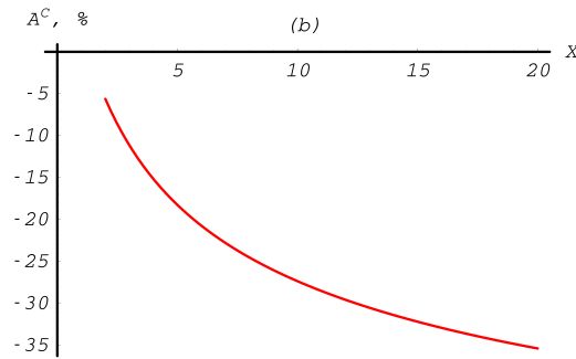
Fig. 14.19: Compton total cross section asymmetry depending on the energy of incoming photon. Up to 10MeV.
