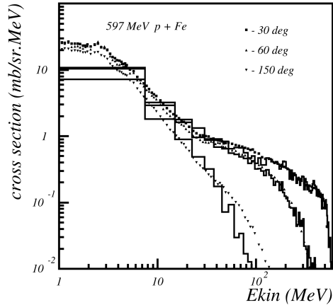
Fig. 26.7: Double differential cross-section for neutrons produced in proton scattering off Iron. Proton incident energy was 597 MeV. The points are data, the histogram is Binary Cascade prediction.
