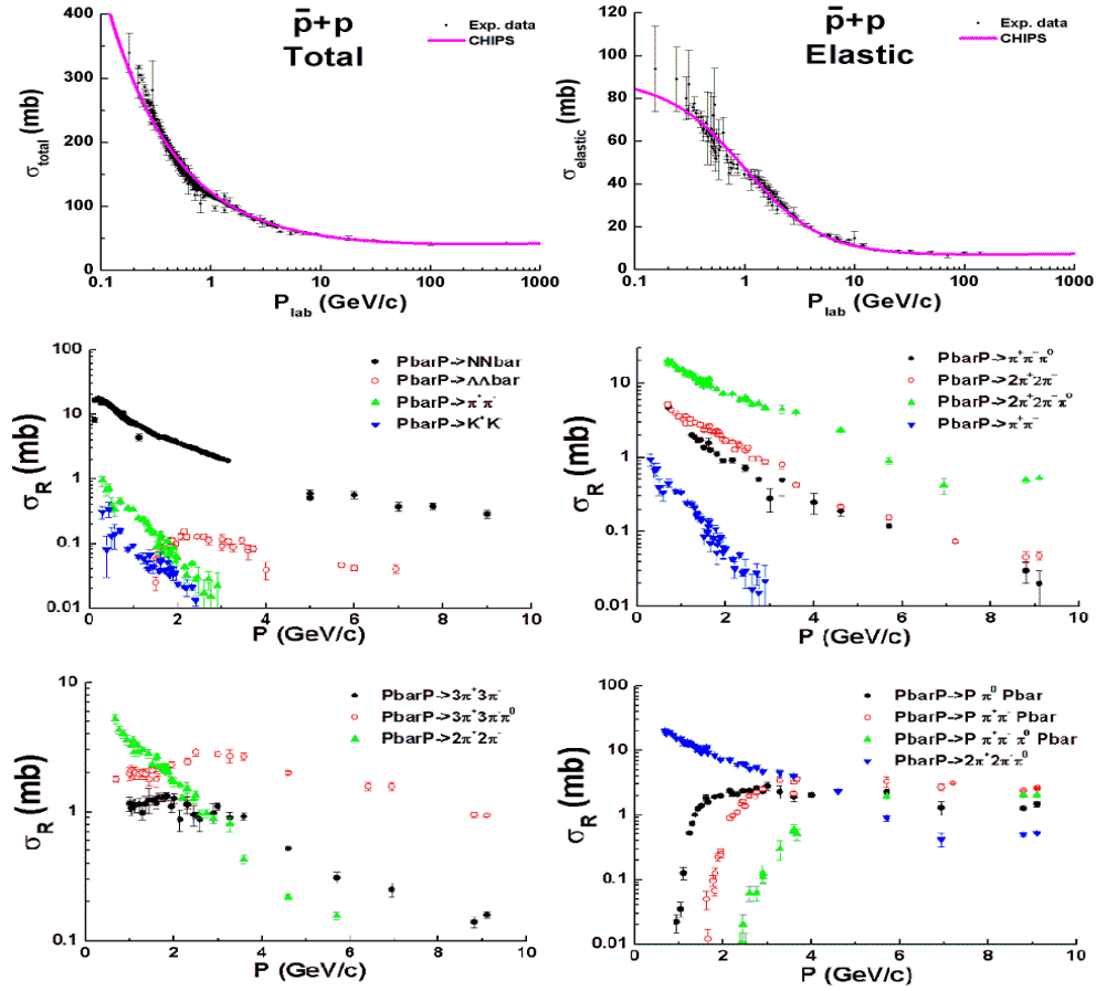
Fig. 24.9: General properties of \bar{p}p -interactions. Points are experimental data: data on total and elastic cross sections from PDG data-base [PDG12], other data from [eal73a, eal84].
