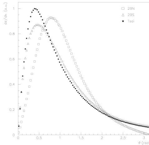
Fig. 11.3: Comparison of polar angle distribution of bremsstrahlung photons ( k/T = 0.5 ) for 100 keV electrons in silver, obtained with Tsai, 2BS and 2BN generator
