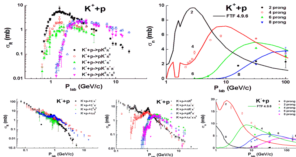
Fig. 24.8: Reaction cross sections of Kp -interactions. Points are experimental data.
