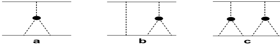
Fig. 24.17: Simplest enhanced diagrams of NN -scattering.
