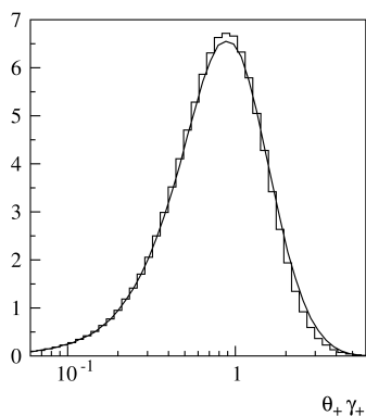
Fig. 7.14: Angular distribution in logarithmic scale. The curve corresponds to the exact calculations and the histogram is the simulated distribution.
