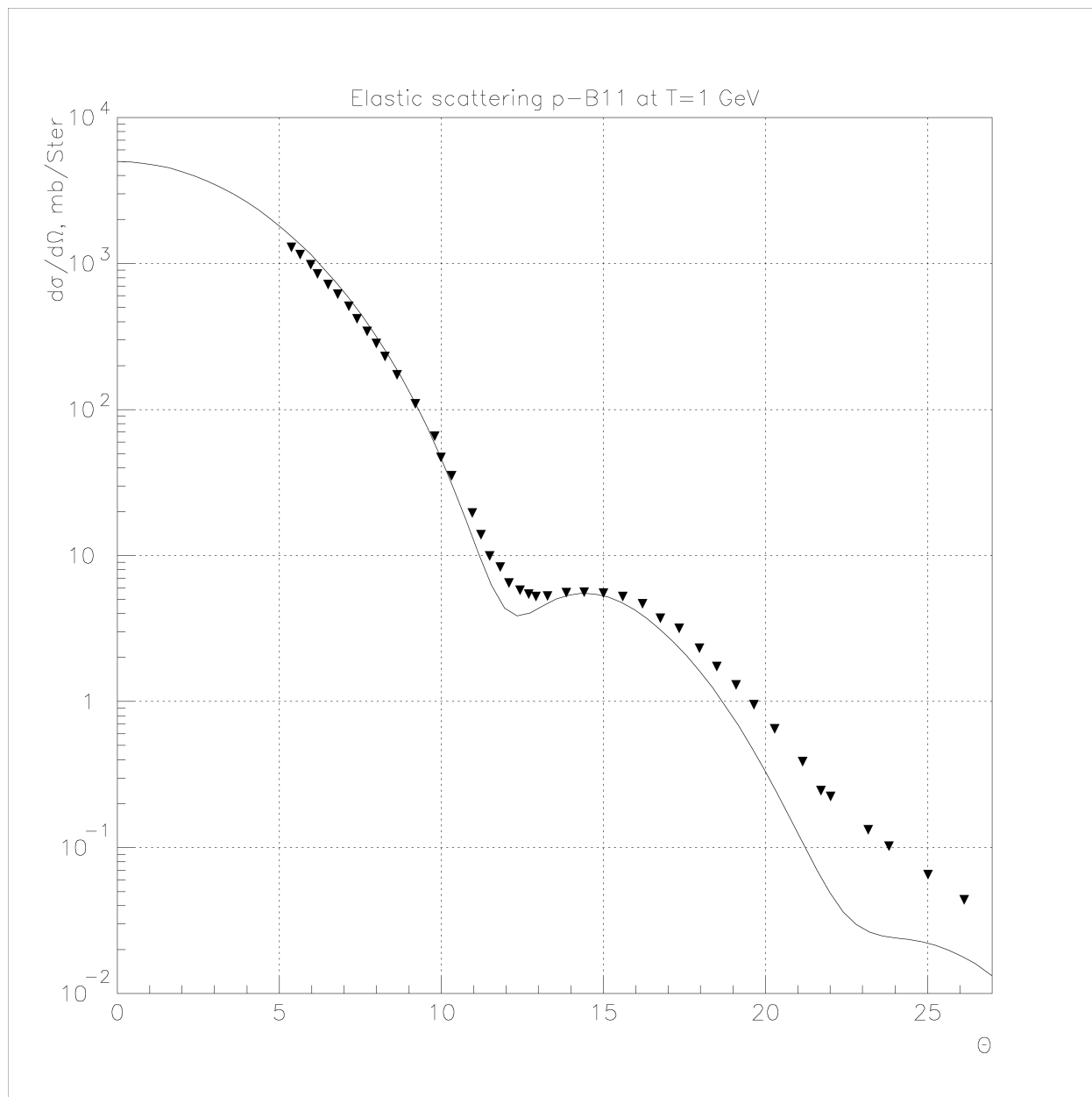
Fig. 22.2: Elastic proton scattering on ^{11}\text{B} at 1 GeV.
