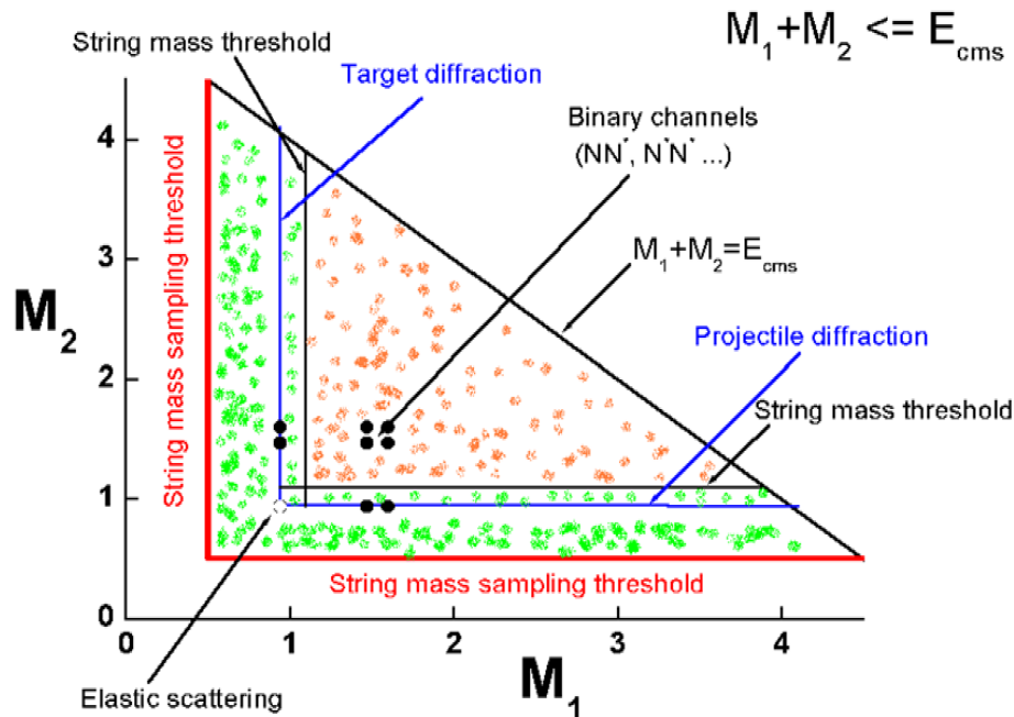
Fig. 24.2: Diagram of the final states of hadron-hadron interactions.
