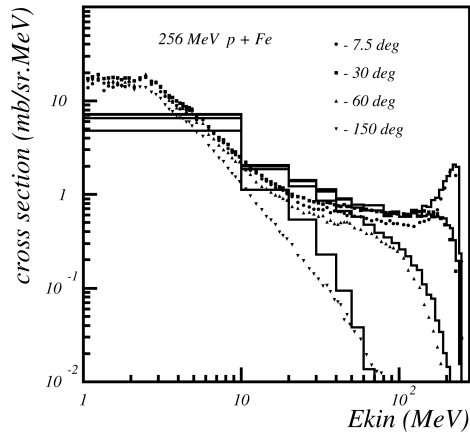
Fig. 26.6: Double differential cross-section for neutrons produced in proton scattering off Iron. Proton incident energy was 256 MeV. The points are data, the histogram is Binary Cascade prediction.
