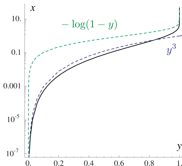
Fig. 15.2: InvSynFracInt on a log x scale. The functions x^{1/3} , y^3 and 1 - e^{-x} , -\log(1 - y) are shown as dashed lines.
