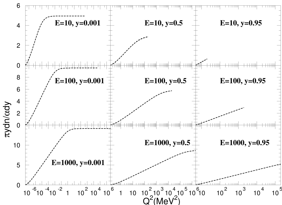
Fig. 43.2: Integrals of Q^2 spectra of virtual photons for three energies 10 MeV, 100 MeV, and 1 GeV at y=0.001 , y=0.5 , and y=0.95 . The solid line corresponds to Eq. (43.3) and the dashed line (which almost everywhere coincides with the solid line) corresponds to Eq. (43.3).
