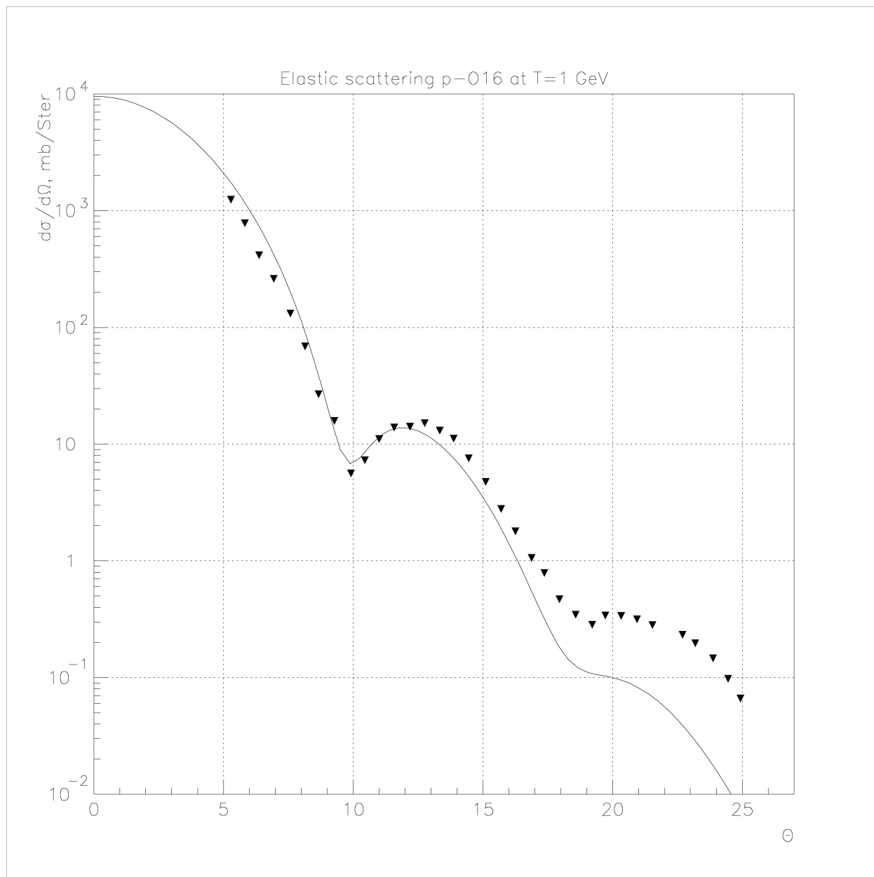
Fig. 22.4: Elastic proton scattering on 16 O at 1 GeV.
