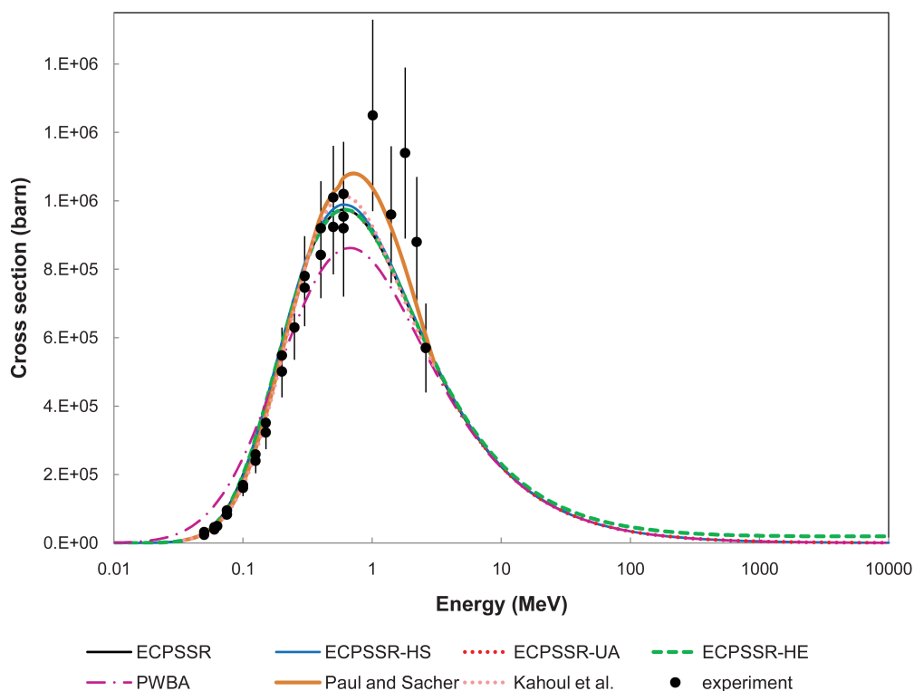
Fig. 10.2: Cross section for the ionisation of carbon K shell by proton impact according to the various implemented modeling options, and comparison with experimental data [PS89]: ECPSSR model, ECPSSR model with “united atom” (UA) approximation, Hartree-Slater (HS) corrections and specialized for high energies (HE); plane wave Born approximation (PWBA); empirical models by Paul and Sacher and Kahoul et al. The curves reproducing some of the model implementations can be hardly distinguished in the plot due to their similarity.
