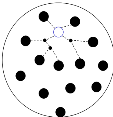
Fig. 24.19: Reggeon "cascade" in hA-scattering.
