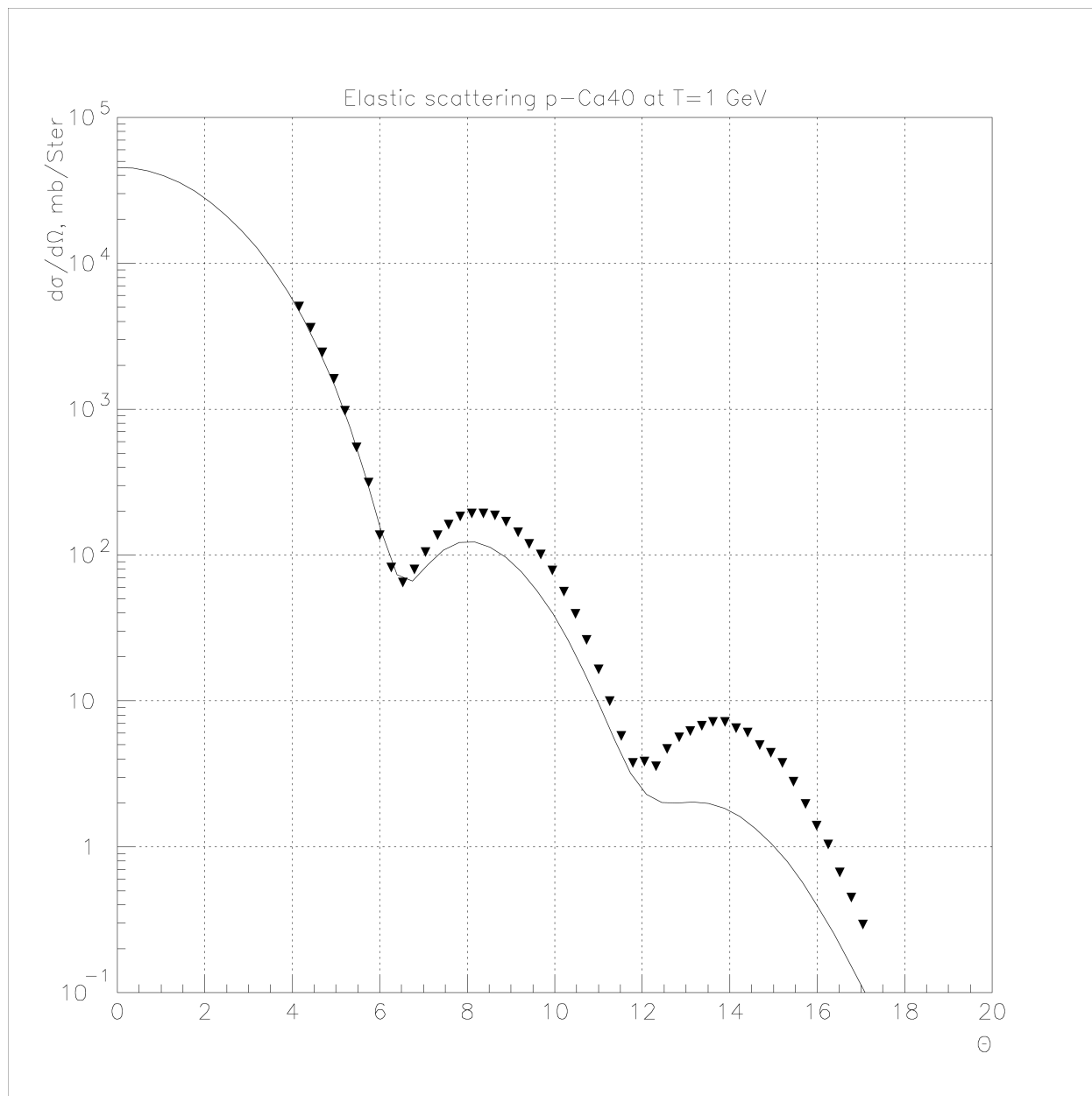
Fig. 22.6: Elastic proton scattering on ^{40}\text{Ca} at 1 GeV.
