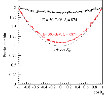
Fig. 11.7: Generated histograms with 10^6 entries each and the expected \cos \theta_{\text{cm}} distributions (dashed lines) at E = 50 and 500 GeV positron energy in the lab frame. The asymptotic 1 + \cos^2 \theta_{\text{cm}} distribution valid for E \rightarrow \infty is shown as dotted line.
