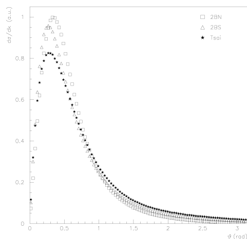
Fig. 11.4: Comparison of polar angle distribution of bremsstrahlung photons ( k/T = 0.5 ) for 500 keV electrons in silver, obtained with Tsai, 2BS and 2BN generator
