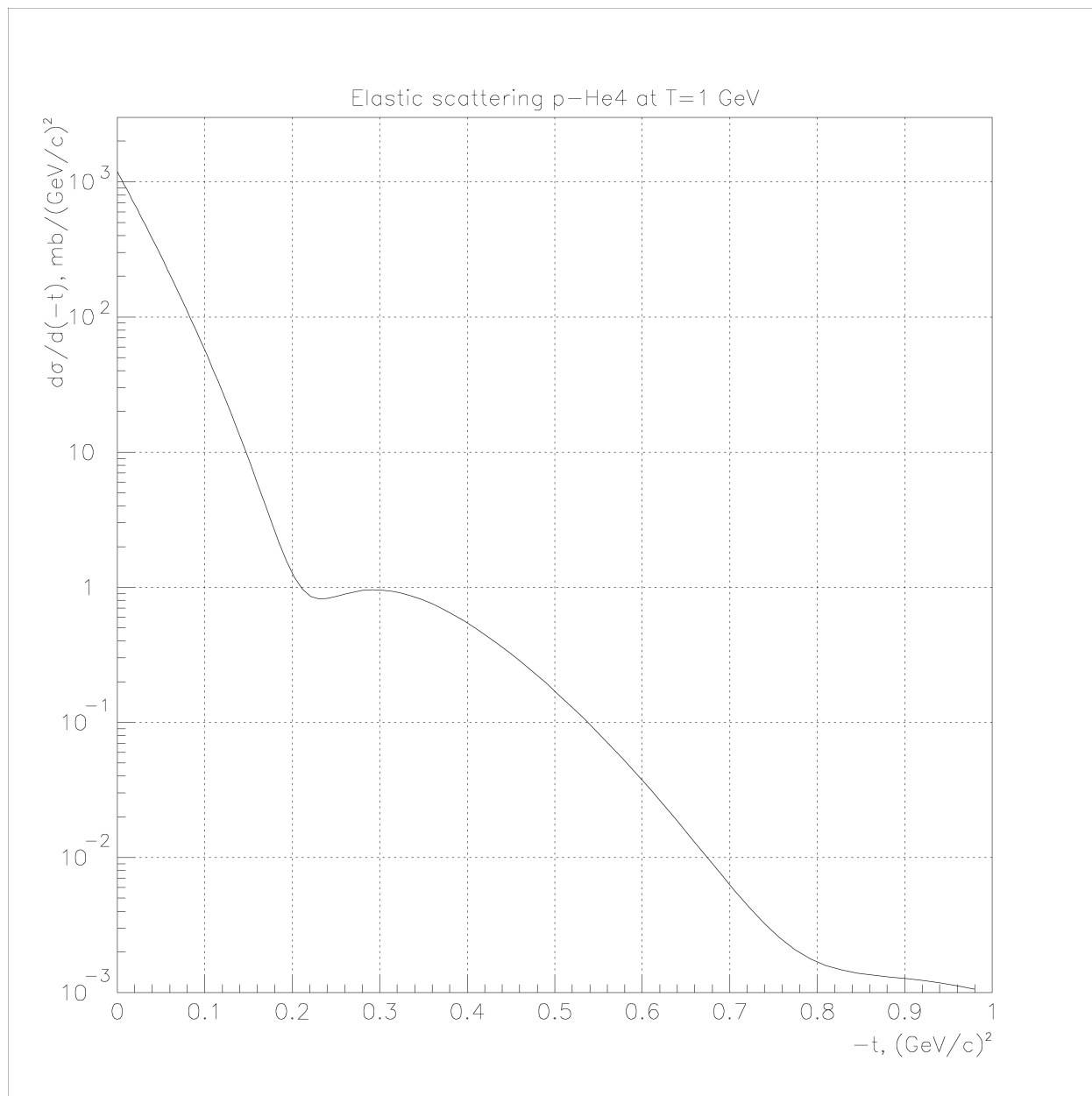
Fig. 22.10: Elastic proton scattering on ^4\text{He} at 1 GeV.
