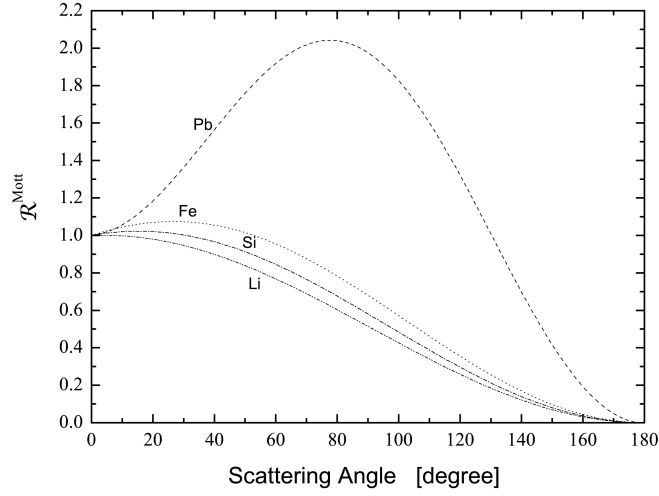
Fig. 9.4: \mathcal{R}^{\text{Mott}} obtained from Eq.(9.48) at 100 MeV for Li, Si, Fe and Pb nuclei as a function of scattering angle.
