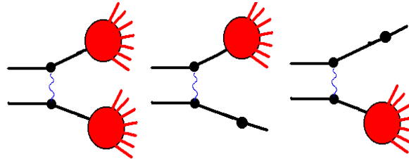
Fig. 24.1: Non-diffractive and diffractive interactions considered in the Fritiof model.
