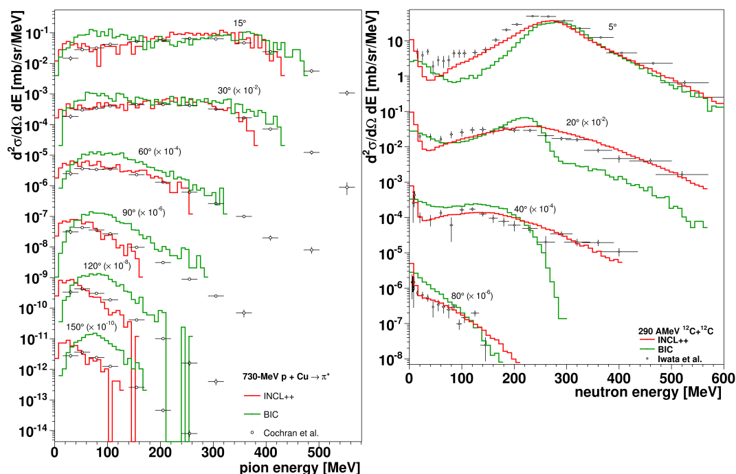
Fig. 27.2: Left: double-differential cross sections for the production of charged pions in 730-MeV p + \text{Cu} . Right: double-differential cross sections for the production of neutrons in 290-AMeV ^{12}\text{C} + ^{12}\text{C} . Predictions of the INCL++ and Binary-Cascade models are compared with experimental data from Refs. [CDG+72] and [IMS+01].
