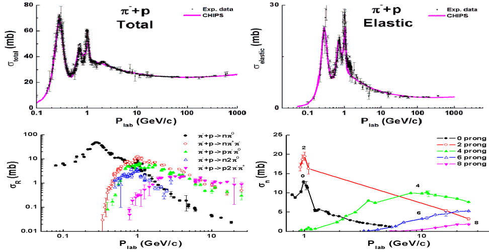
Fig. 24.3: General properties of \pi^-p -interactions. Points are experimental data: data on total and elastic cross sections from PDG data-base [PDG12], other data from [eal72].
