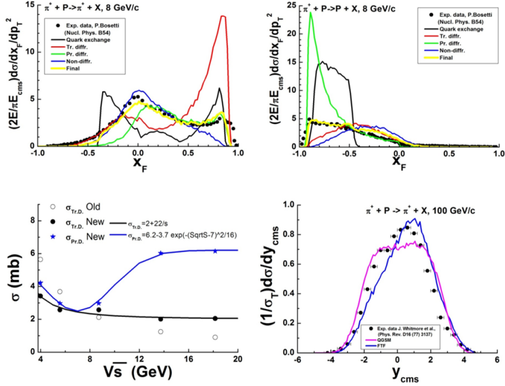
Fig. 24.12: Upper figures: inclusive spectra of protons and \pi^+ -mesons in \pi^+ p -interactions. Points are experimental data [eal73b]. Lines represent the contributions of the various FTF processes calculated by assuming that the probability of each process is 100 %. Bottom left figure: diffraction dissociation cross sections obtained by tuning (points), and their description (lines) by the expression for \pi in (24.4). Bottom right figure: rapidity spectrum of \pi^+ -mesons in \pi^+ p -interactions at p_{\text{lab}} = 100 GeV/c. Points are experimental data [Whi74].
