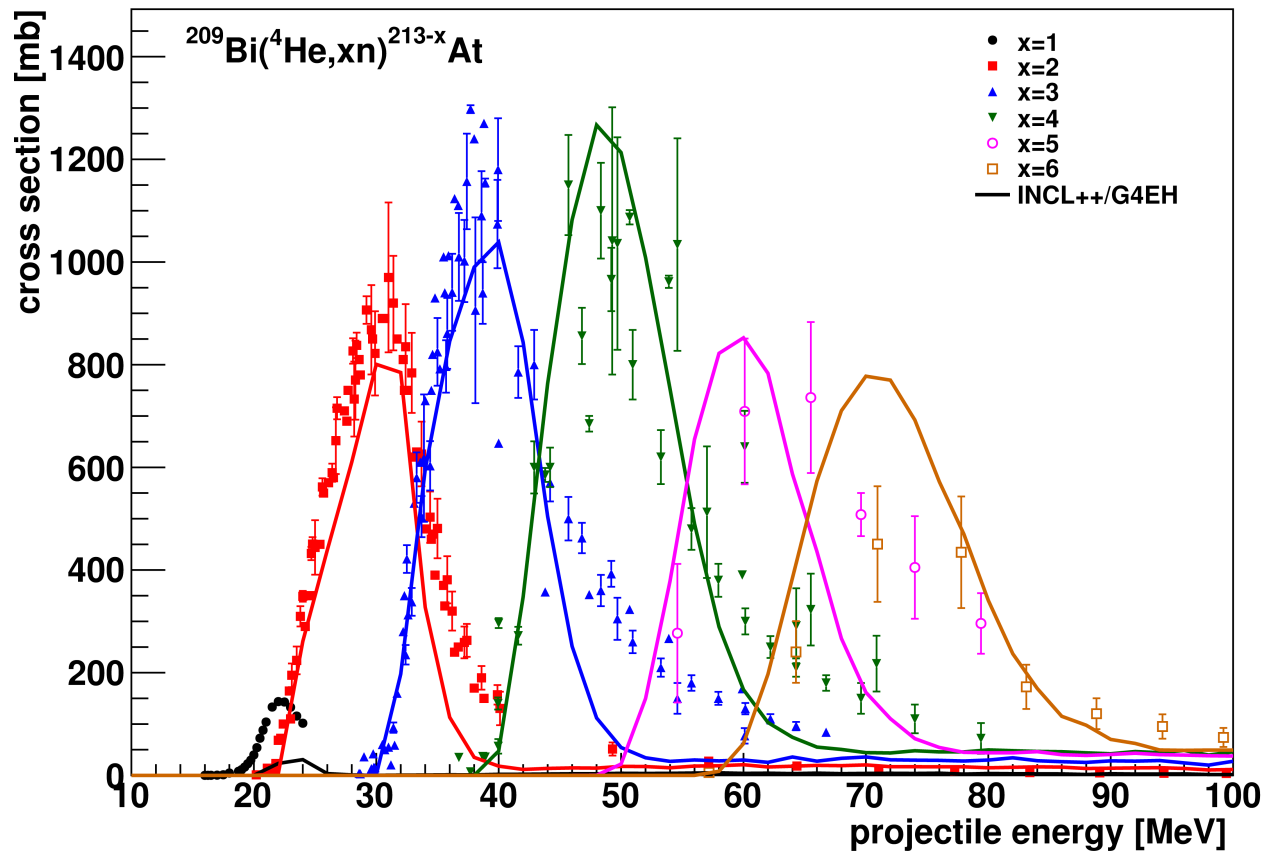
Fig. 27.3: Excitation functions for (\alpha, xn) cross sections on ^{209}\text{Bi} . The predictions of INCL++-G4ExcitationHandler are represented by the solid line and are compared to experimental data [BL74, DL74, eal05, KSegre49, LM85, RBAC90, SMS94, SH74, PatelShahSingh99].
