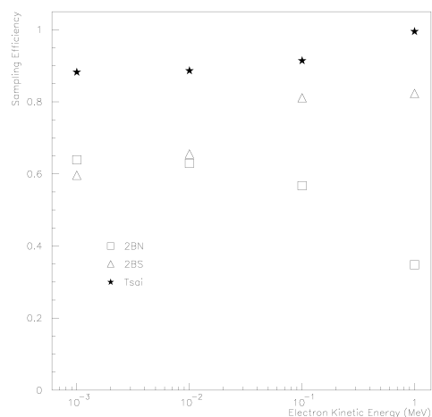
Fig. 11.5: Sampling efficiency for Tsai generator, 2BS and 2BN Koch and Motz generators.
