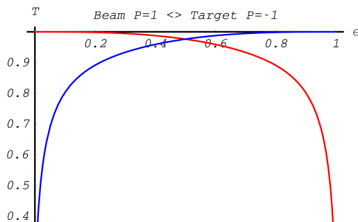
Fig. 14.9: Polarization transfer functions in Møller scattering. Longitudinal polarization \xi_3^{(2)} of electron with energy E_{p_2} in blue; longitudinal polarization \xi_3^{(1)} of second electron in red. Kinetic energy of incoming electron T_{k_1} = 10\text{MeV}
