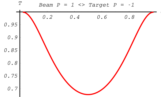
Fig. 14.17: Polarization Transfer in annihilation process. Blue line corresponds to the circular polarization \xi_3^{(1)} of the photon with energy m(\gamma + 1)\epsilon ; red line – circular polarization \xi_3^{(2)} of the photon with energy m(\gamma + 1)(1 - \epsilon) .
