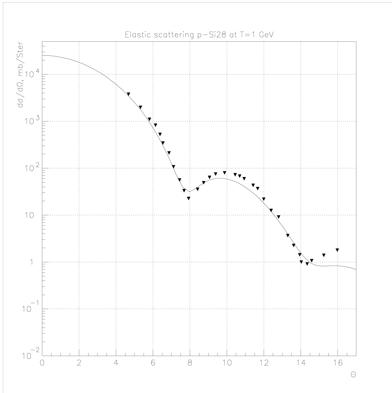
Fig. 22.5: Elastic proton scattering on ^{28}\text{Si} at 1 GeV.
