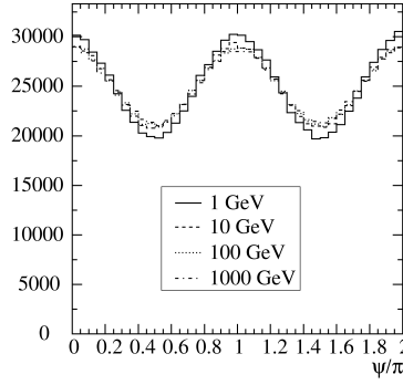
Fig. 7.10: Histograms of generated \psi distributions for beryllium at four different photon energies.
