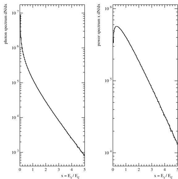
Fig. 15.3: Comparison of the exact (smooth curve) and generated (histogram) spectra for 2 \times 10^7 events. The photon spectrum is shown on the left and the power spectrum on the right side.
