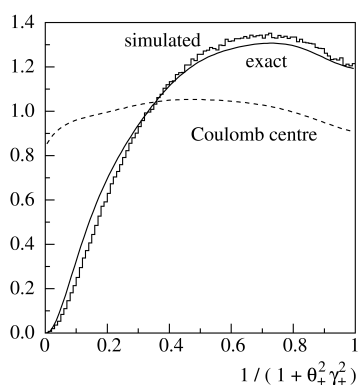
Fig. 7.13: Angular distribution of positive (or negative) muons. The solid curve represents the results of the exact calculations. The histogram is the simulated distribution. The angular distribution for pairs created in the field of the Coulomb centre (point-like target) is shown by the dashed curve for comparison.
