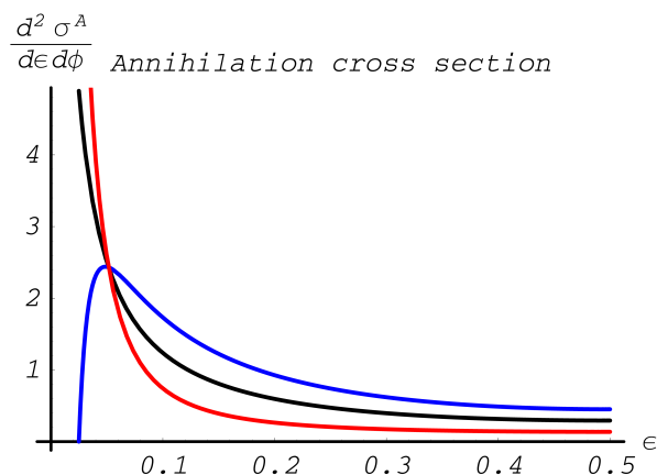
Fig. 14.14: Annihilation differential cross section in arbitrary units. Black line corresponds to unpolarized cross section; red line – to the antiparallel spins of initial particles, and blue line – to the parallel spins. Kinetic energy of the incoming positron T_{k_1} = 10\text{MeV} .
