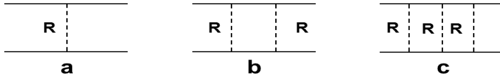
Fig. 24.16: Nonenhanced diagrams of NN -scattering.
