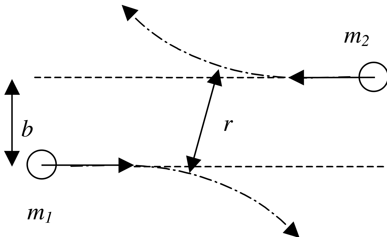
Fig. 35.2: Illustration clarifying impact parameter in the far-field ( b ) and actual impact parameter ( r ).
