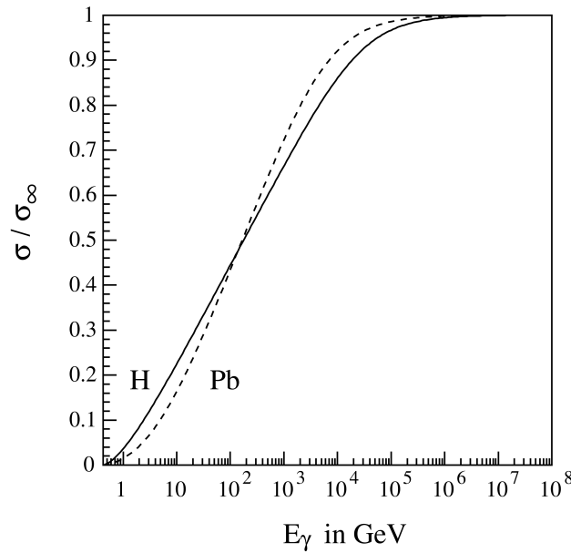
Fig. 7.4: Total cross section for the Bethe-Heitler process \gamma \rightarrow \mu^+ \mu^- as a function of the photon energy E_\gamma in hydrogen and lead, normalized to the asymptotic cross section \sigma_\infty .
