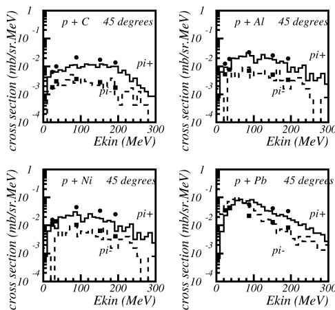
Fig. 26.13: Double differential cross-section for pions produced at 45^\circ in proton scattering off various materials. Proton incident energy was 597 MeV in each case. The points are data, the histogram is Binary Cascade prediction.
