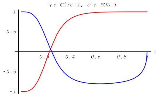
Fig. 14.22: Polarization Transfer in Compton scattering. Blue line corresponds to the longitudinal polarization \xi_3^{(2)} of the electron, red line – circular polarization \xi_3^{(1)} of the photon.
