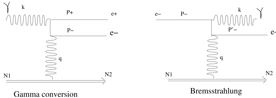
Fig. 14.24: Feynman diagrams of Gamma conversion and bremsstrahlung processes.
