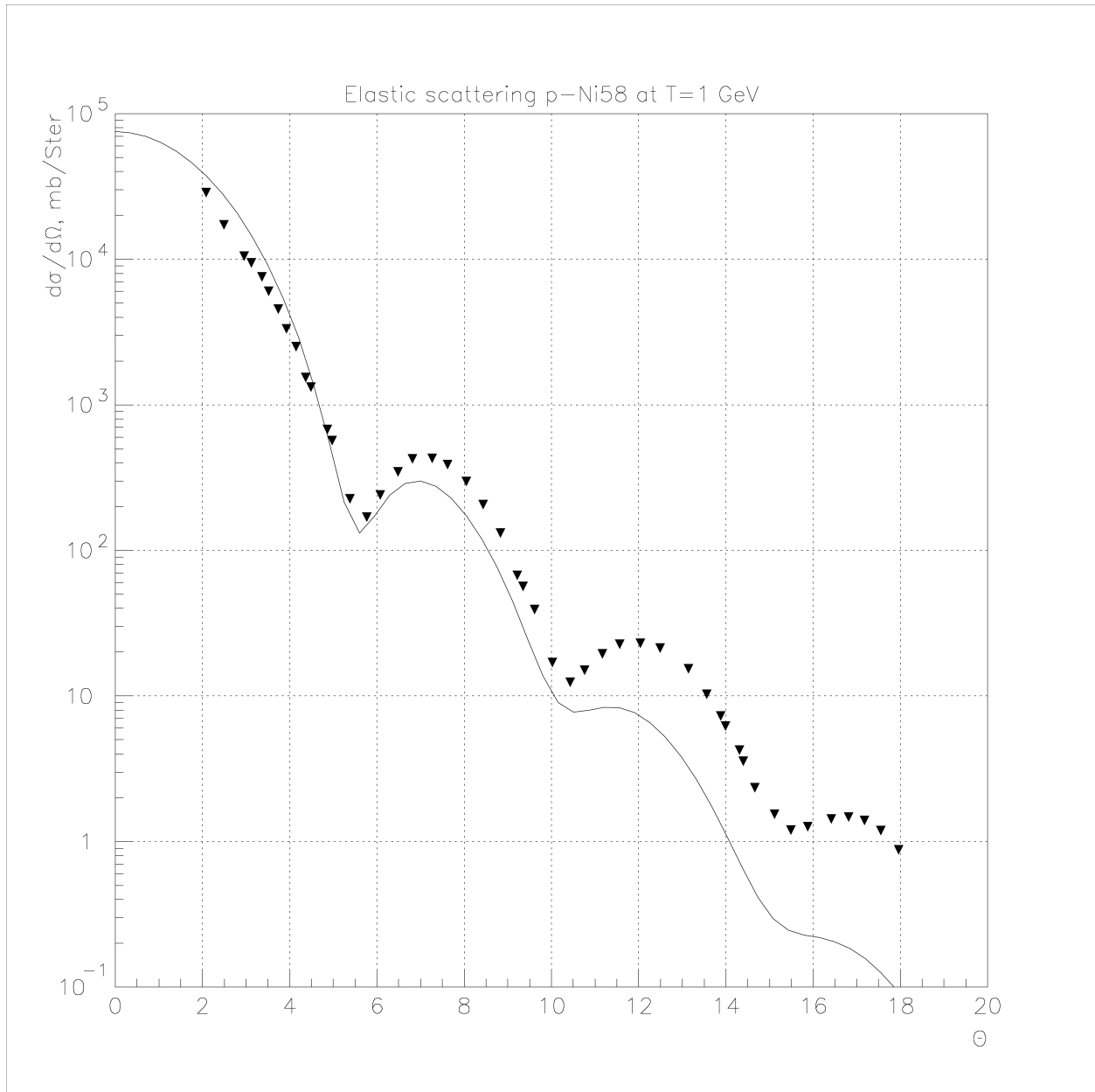
Fig. 22.7: Elastic proton scattering on ^{58}\text{Ni} at 1 GeV.
