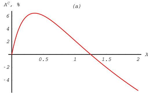
Fig. 14.18: Compton total cross section asymmetry depending on the energy of incoming photon. Between 0 and \sim 1 MeV.
