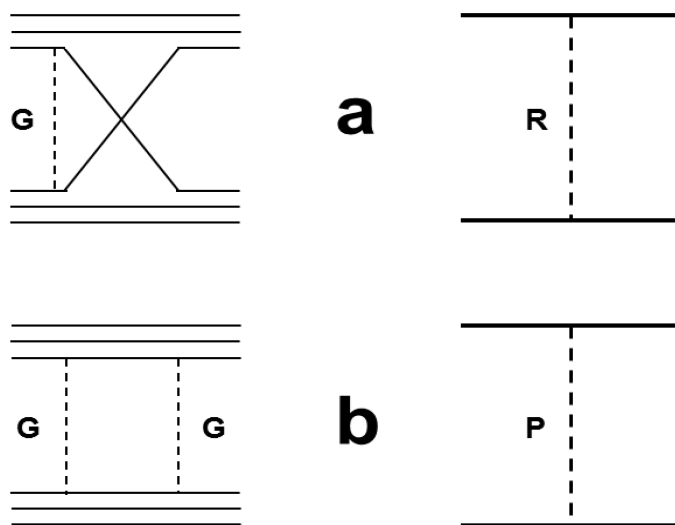
Fig. 24.20: Diagrams of quark-gluon exchanges and corresponding reggeon diagrams for hadron-nucleus interactions.
