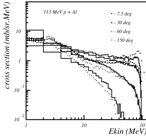
Fig. 26.1: Double differential cross-section for neutrons produced in proton scattering off Aluminum. Proton incident energy was 113 MeV.
