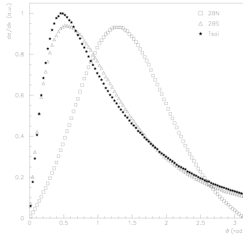
Fig. 11.2: Comparison of polar angle distribution of bremsstrahlung photons ( k/T = 0.5 ) for 10 keV electrons in silver, obtained with Tsai, 2BS and 2BN generator
