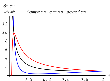
Fig. 14.20: Compton scattering differential cross section in arbitrary units. Black line corresponds to the unpolarized cross section; red line – to the antiparallel spins of initial particles, and blue line – to the parallel spins. Energy of the incoming photon E_{k_1} = 10\text{MeV} .
