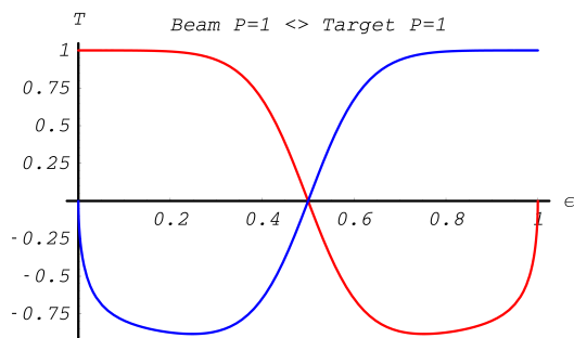
Fig. 14.8: Polarization transfer functions in Møller scattering. Longitudinal polarization \xi_3^{(2)} of electron with energy E_{p_2} in blue; longitudinal polarization \xi_3^{(1)} of second electron in red. Kinetic energy of incoming electron T_{k_1} = 10\text{MeV}
