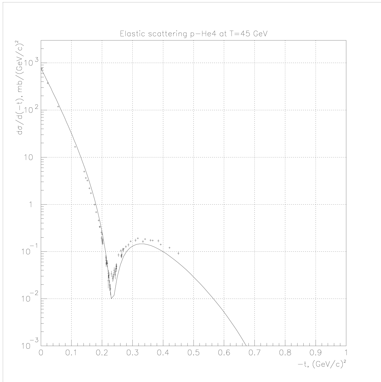
Fig. 22.11: Elastic proton scattering on ^4\text{He} at 45 GeV.
