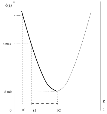
Fig. 7.2: Calculation of \epsilon for gamma conversion.
