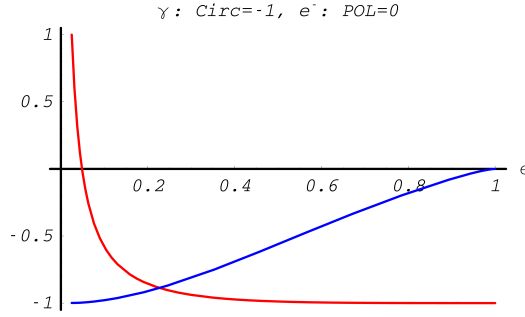
Fig. 14.23: Polarization Transfer in Compton scattering. Blue line corresponds to the longitudinal polarization \xi_3^{(2)} of the electron, red line – circular polarization \xi_3^{(1)} of the photon.
