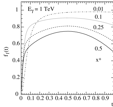
Fig. 7.8: The function f_1(t) at E_\gamma = 1 TeV in beryllium for different values of x_+ .
