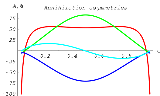
Fig. 14.15: Annihilation differential cross section asymmetries in %. Red line corresponds to A_{ZZ}(\epsilon) , green line – A_{XX}(\epsilon) , blue line – A_{YY}(\epsilon) , lightblue line – A_{ZX}(\epsilon) . Kinetic energy of the incoming positron T_{k_1} = 10\text{MeV} .
