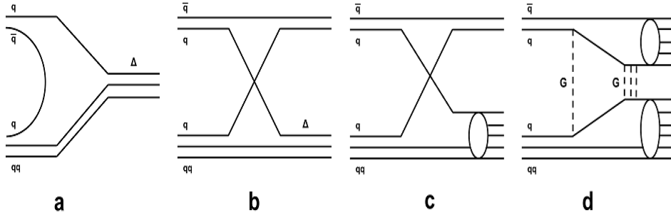
Fig. 24.4: Quark flow diagrams of \pi N -interactions.
