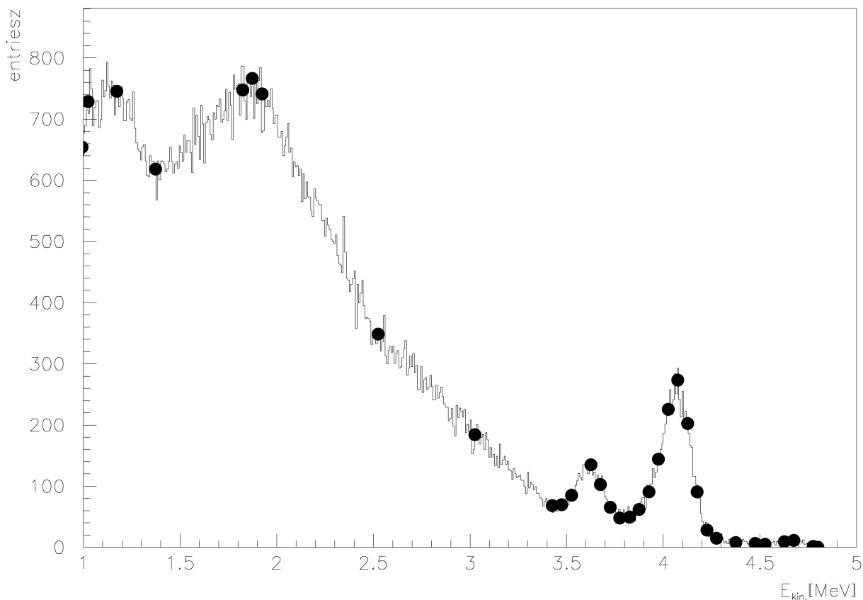
Fig. 38.2: Comparison of data and Monte Carlo for photon energy distributions for radiative capture of 15 MeV neutrons on Uranium ( ^{238}\text{U} ). The points are evaluated data, the histogram is the Monte Carlo prediction.
