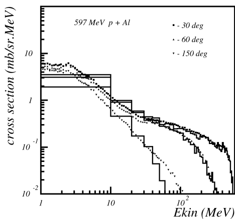
Fig. 26.3: Double differential cross-section for neutrons produced in proton scattering off Aluminum. Proton incident energy was 597 MeV. The points are data, the histogram is Binary Cascade prediction.
