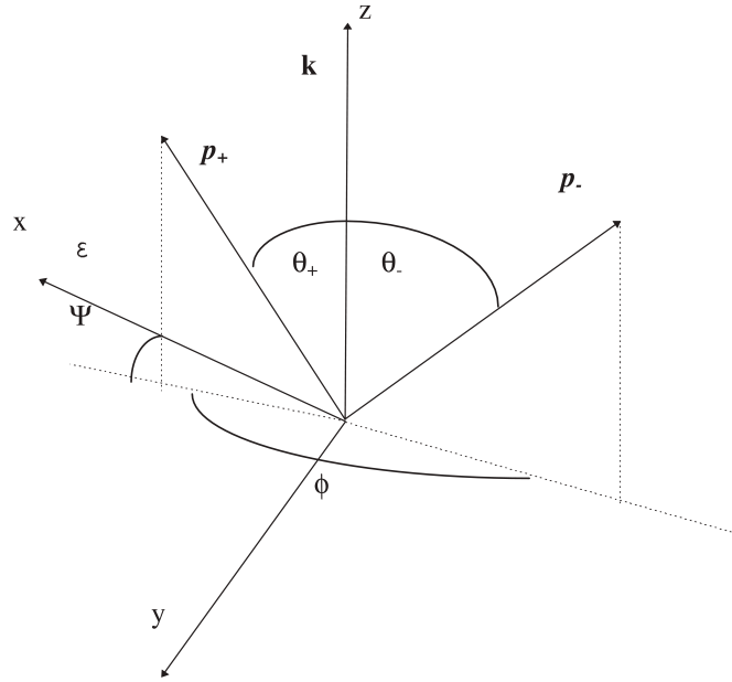
Fig. 14.25: Angles occurring in the pair creation
