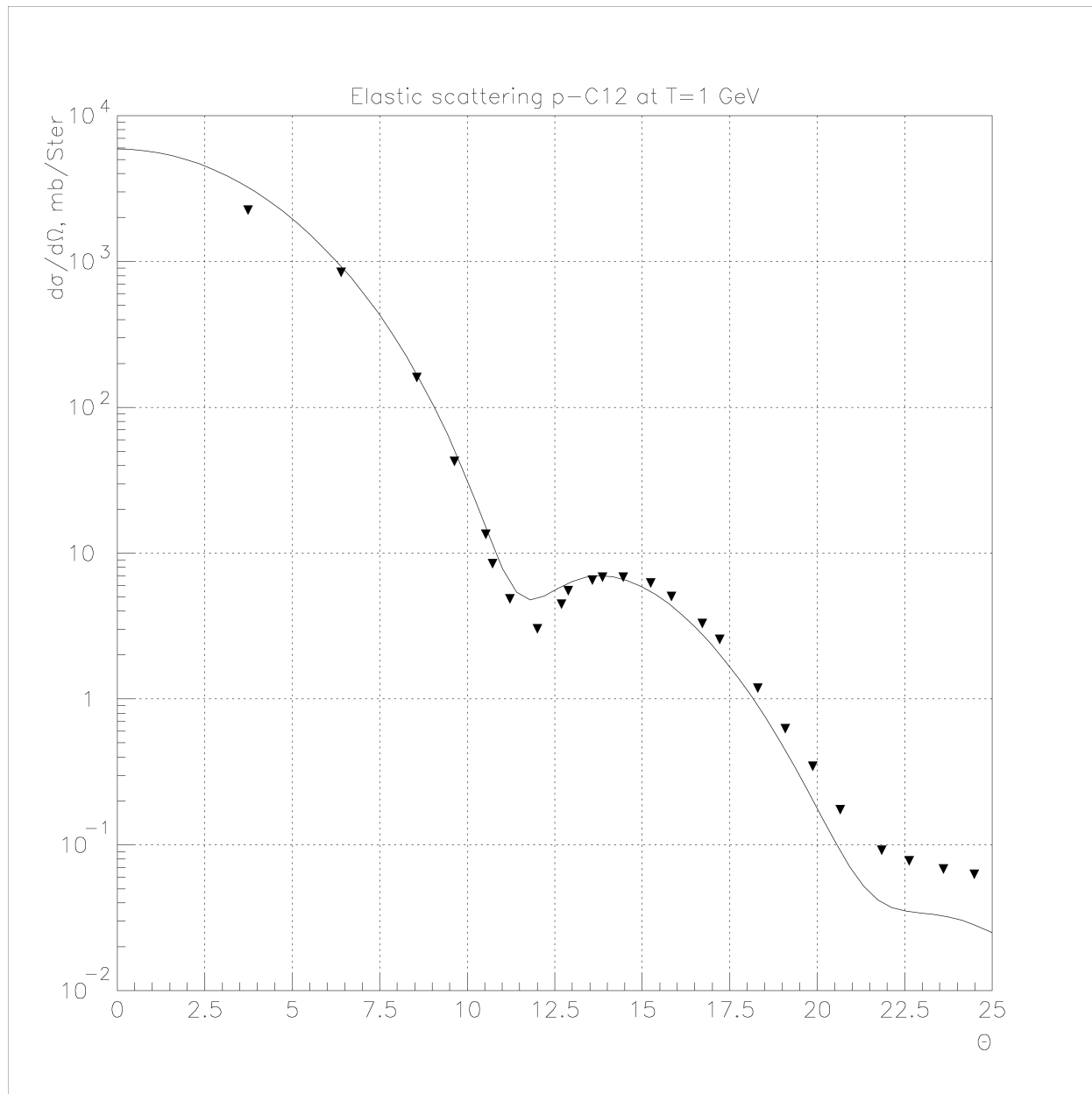
Fig. 22.3: Elastic proton scattering on ^{12}\text{C} at 1 GeV.
