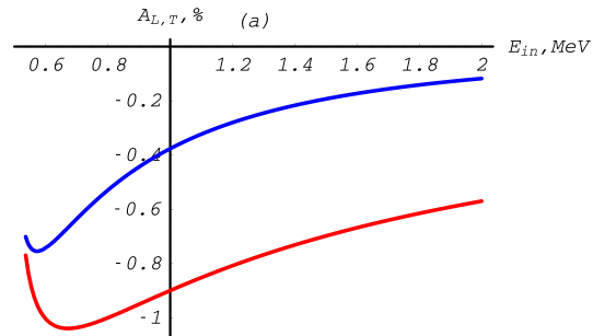
Fig. 14.4: Bhabha total cross section asymmetries depending on the total energy of the incoming positron, with a cut-off T_{\text{cut}} = 1\text{keV} . Transverse asymmetry is plotted in blue, longitudinal asymmetry in red. Between 0.5 MeV and 2 MeV.
