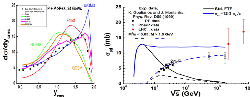
Fig. 24.11: Left: inclusive spectrum of proton in pp -interactions at P_{lab} = 24 GeV/c. Points are experimental data [eal74], lines are model calculations. Right: single diffraction dissociation cross section in pp -interactions. Points are data gathered by K. Goulianos and J. Montanha [GM99]. Lines are FTF model calculations.
