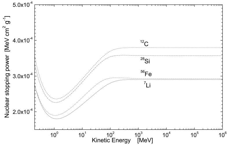
Fig. 9.5: In \text{MeV cm}^2/\text{g} , nuclear stopping powers in {}^7\text{Li} , {}^{12}\text{C} , {}^{28}\text{Si} and {}^{56}\text{Fe} calculated from Eq.(9.75) and divided by the density of the material as a function of the kinetic energy of electrons from 200 keV up to 1 TeV.
