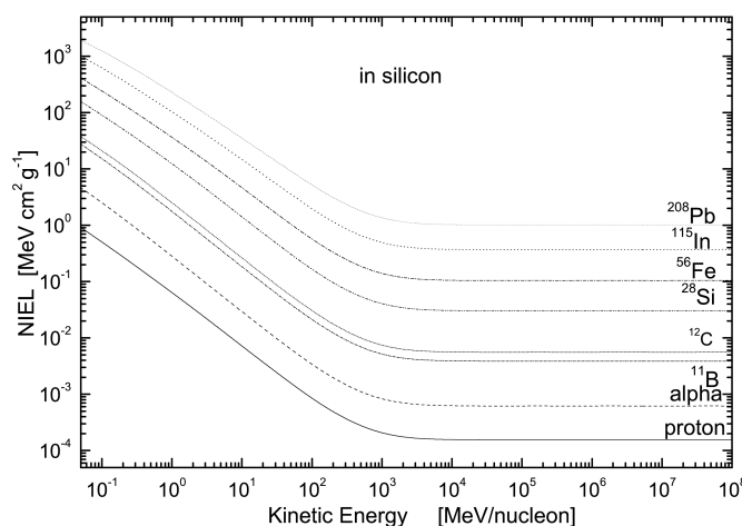
Fig. 9.3: Non-ionizing stopping power from Ref. [eal11] calculated using Eq.(9.33) in silicon is shown as a function of the kinetic energy per nucleon, from 50 keV/nucleon up 100 TeV/nucleon, for protons, \alpha -particles and ^{11}\text{B} , ^{12}\text{C} , ^{28}\text{Si} , ^{56}\text{Fe} , ^{115}\text{In} , ^{208}\text{Pb} nuclei. The threshold energy for displacement is 21 eV in silicon.
