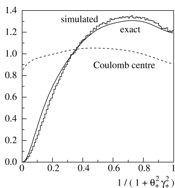
Fig. 6.13: Angular distribution of positive (or negative) muons. The solid curve represents the results of the exact calculations. The histogram is the simulated distribution. The angular distribution for pairs created in the field of the Coulomb centre (point-like target) is shown by the dashed curve for comparison.
