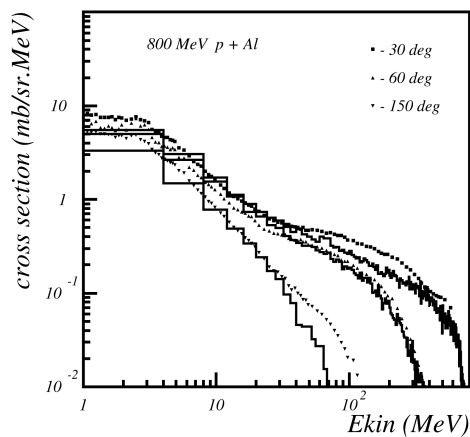
Fig. 27.4: Double differential cross-section for neutrons produced in proton scattering off Aluminum. Proton incident energy was 800 MeV. The points are data, the histogram is Binary Cascade prediction.
