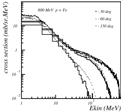
Fig. 27.8: Double differential cross-section for neutrons produced in proton scattering off Iron. Proton incident energy was 800 MeV. The points are data, the histogram is Binary Cascade prediction.
