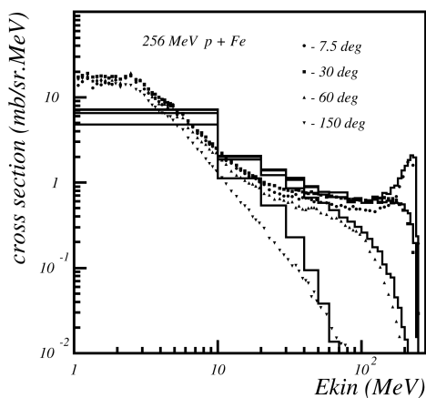
Fig. 27.6: Double differential cross-section for neutrons produced in proton scattering off Iron. Proton incident energy was 256 MeV. The points are data, the histogram is Binary Cascade prediction.
