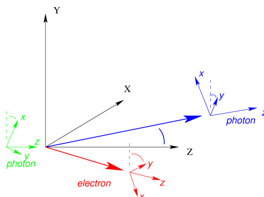
Fig. 13.1: The interaction frame and the particle frames for the example of Compton scattering. The momenta of all participating particle lie in the x - z -plane, the scattering plane. The incoming photon gives the z direction. The outgoing photon is defined as particle 1 and gives the x -direction, perpendicular to the z -axis. The y -axis is then perpendicular to the scattering plane and completes the definition of a right handed coordinate system called interaction frame . The particle frame is defined by the GEANT4 routine G4ThreeMomentum::rotateUz() .
