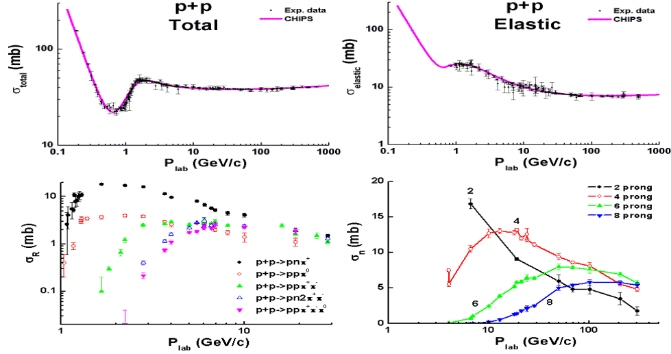
Fig. 25.6: General properties of pp -interactions. Points are experimental data: data on total and elastic cross sections from PDG data-base [PDG12], other data from [eal73a][eal84].
