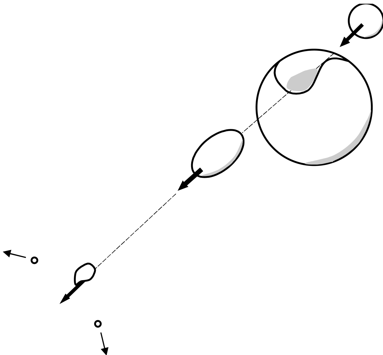
Fig. 36.1: In the abrasion process, a fraction of the nucleons in the projectile and target nucleons interact to form a fireball region with a velocity between that of the projectile and the target. The remaining spectator nucleons in the projectile and target are not initially affected (although they do suffer change as a result of longer-term de-excitation).
