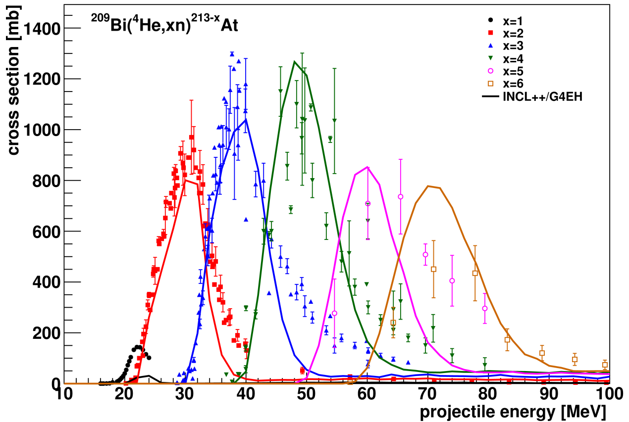
Fig. 28.3: Excitation functions for (\alpha, xn) cross sections on ^{209}\text{Bi} . The predictions of INCL++-G4ExcitationHandler are represented by the solid line and are compared to experimental data [eal05][BL74][KSegre49][DL74][PatelShahSingh99][RBAC90][SH74][SMS94][LM85].
