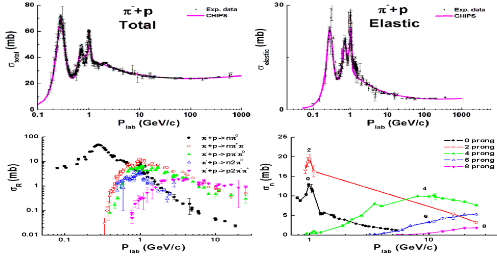
Fig. 25.3: General properties of \pi^-p -interactions. Points are experimental data: data on total and elastic cross sections from PDG data-base [PDG12], other data from [eal72].
