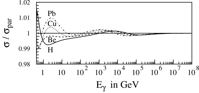
Fig. 6.5: Ratio of numerically integrated and parametrized total cross sections as a function of E_\gamma for hydrogen, beryllium, copper and lead.
