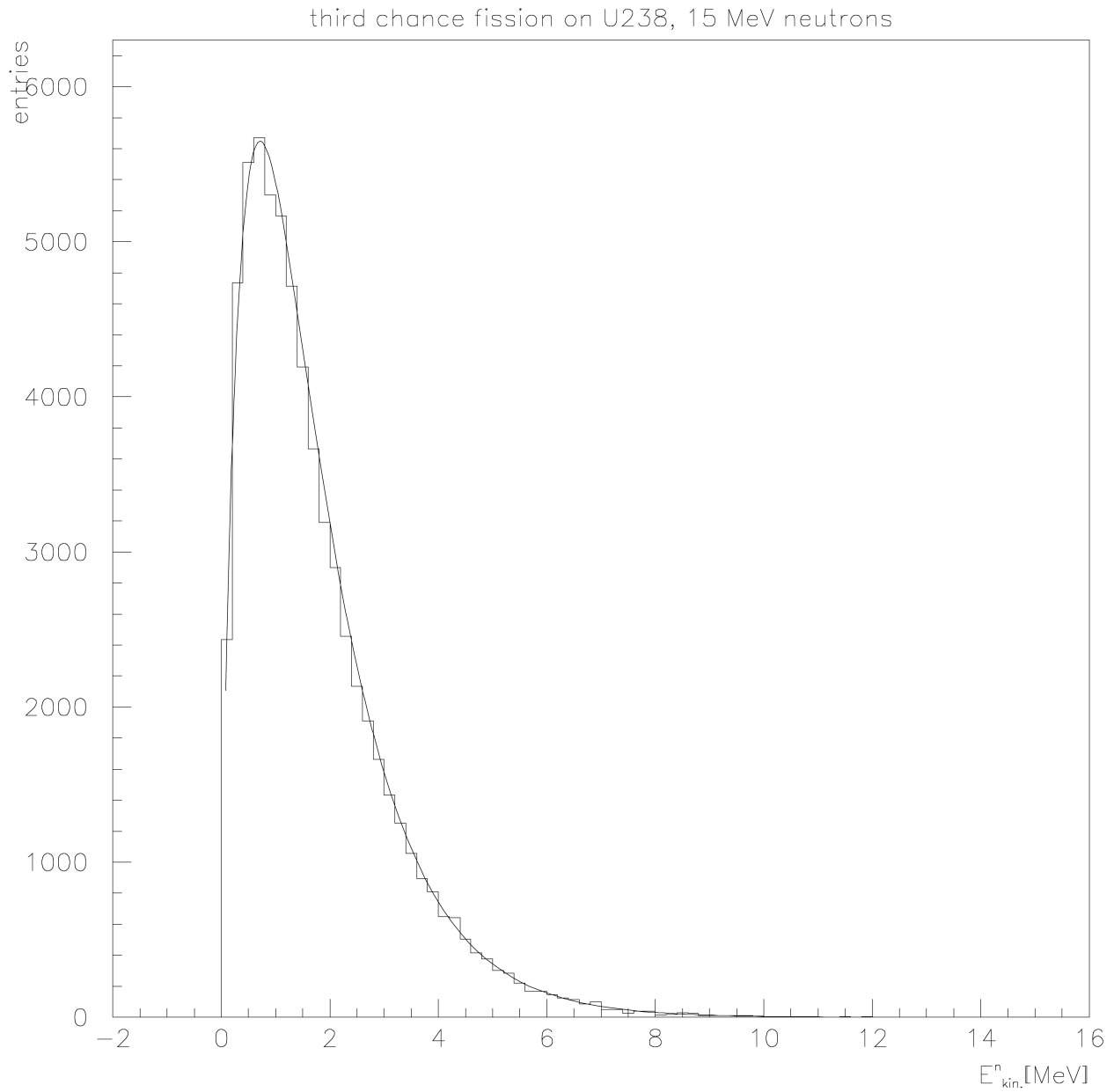
Fig. 39.3: Comparison of data and Monte Carlo for fission neutron energy distributions for induced fission by 15 MeV neutrons on uranium ( ^{238}\text{U} ). The curve represents evaluated data and the histogram is the Monte Carlo prediction.
