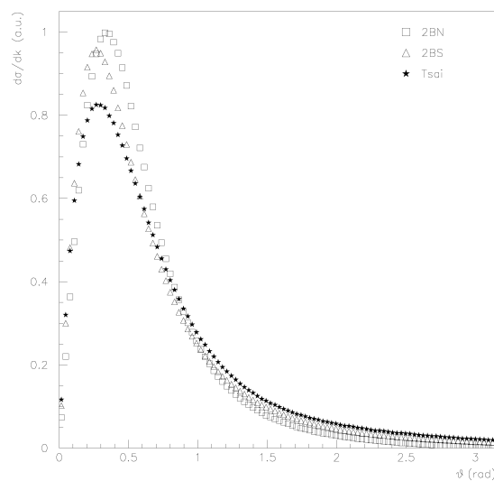
Fig. 10.4: Comparison of polar angle distribution of bremsstrahlung photons ( k/T = 0.5 ) for 500 keV electrons in silver, obtained with Tsai, 2BS and 2BN generator
