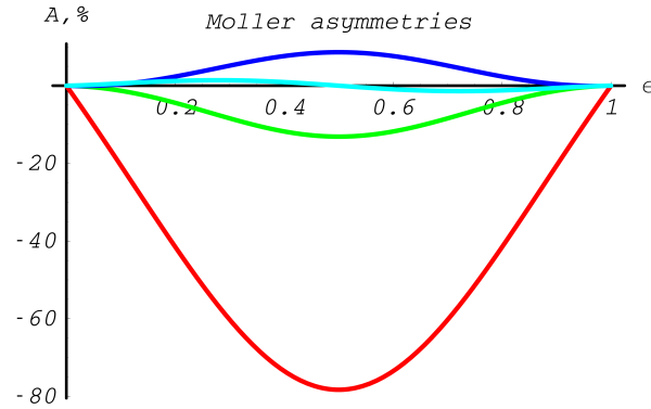
Fig. 13.6: Differential cross section asymmetries in % for Møller scattering (red - A_{ZZ}(\epsilon) , green - A_{XX}(\epsilon) , blue - A_{YY}(\epsilon) , light blue - A_{ZX}(\epsilon) )
