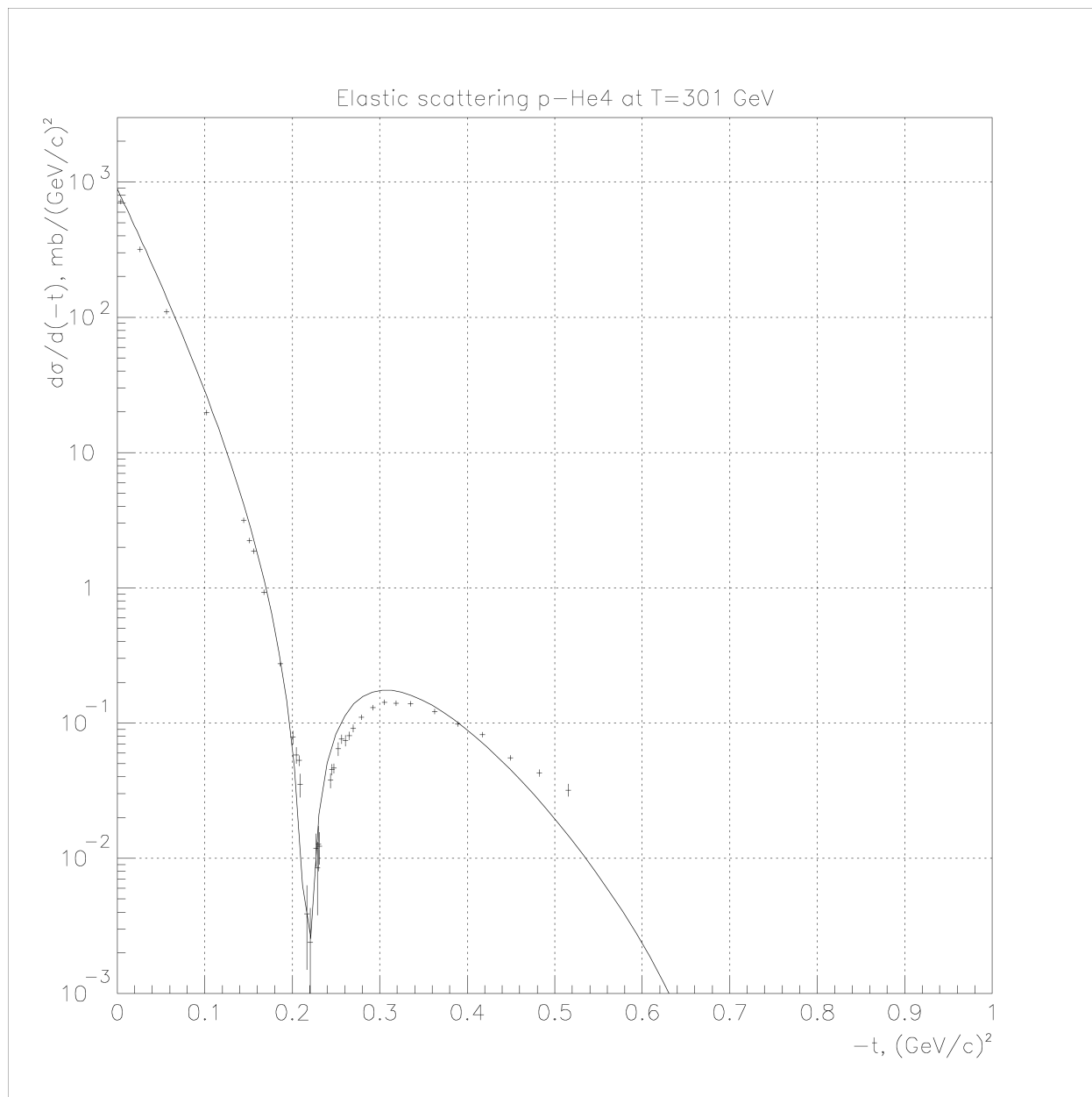
Fig. 23.12: Elastic proton scattering on ^4\text{He} at 301 GeV.
