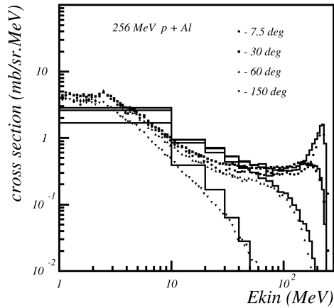
Fig. 27.2: Double differential cross-section for neutrons produced in proton scattering off Aluminum. Proton incident energy was 256 MeV. The points are data, the histogram is Binary Cascade prediction.
