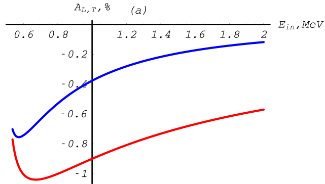
Fig. 13.4: Bhabha total cross section asymmetries depending on the total energy of the incoming positron, with a cut-off T_{\text{cut}} = 1\text{keV} . Transverse asymmetry is plotted in blue, longitudinal asymmetry in red. Between 0.5 MeV and 2 MeV.
