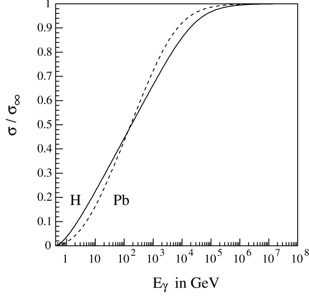
Fig. 6.4: Total cross section for the Bethe-Heitler process \gamma \rightarrow \mu^+ \mu^- as a function of the photon energy E_\gamma in hydrogen and lead, normalized to the asymptotic cross section \sigma_\infty .
