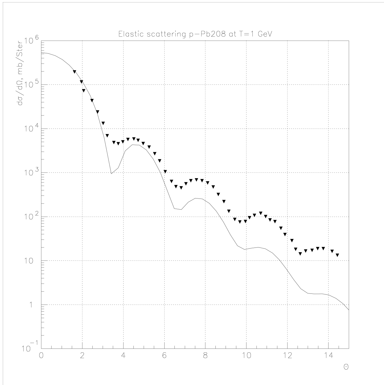
Fig. 23.9: Elastic proton scattering on ^{208}\text{Pb} at 1 GeV.
