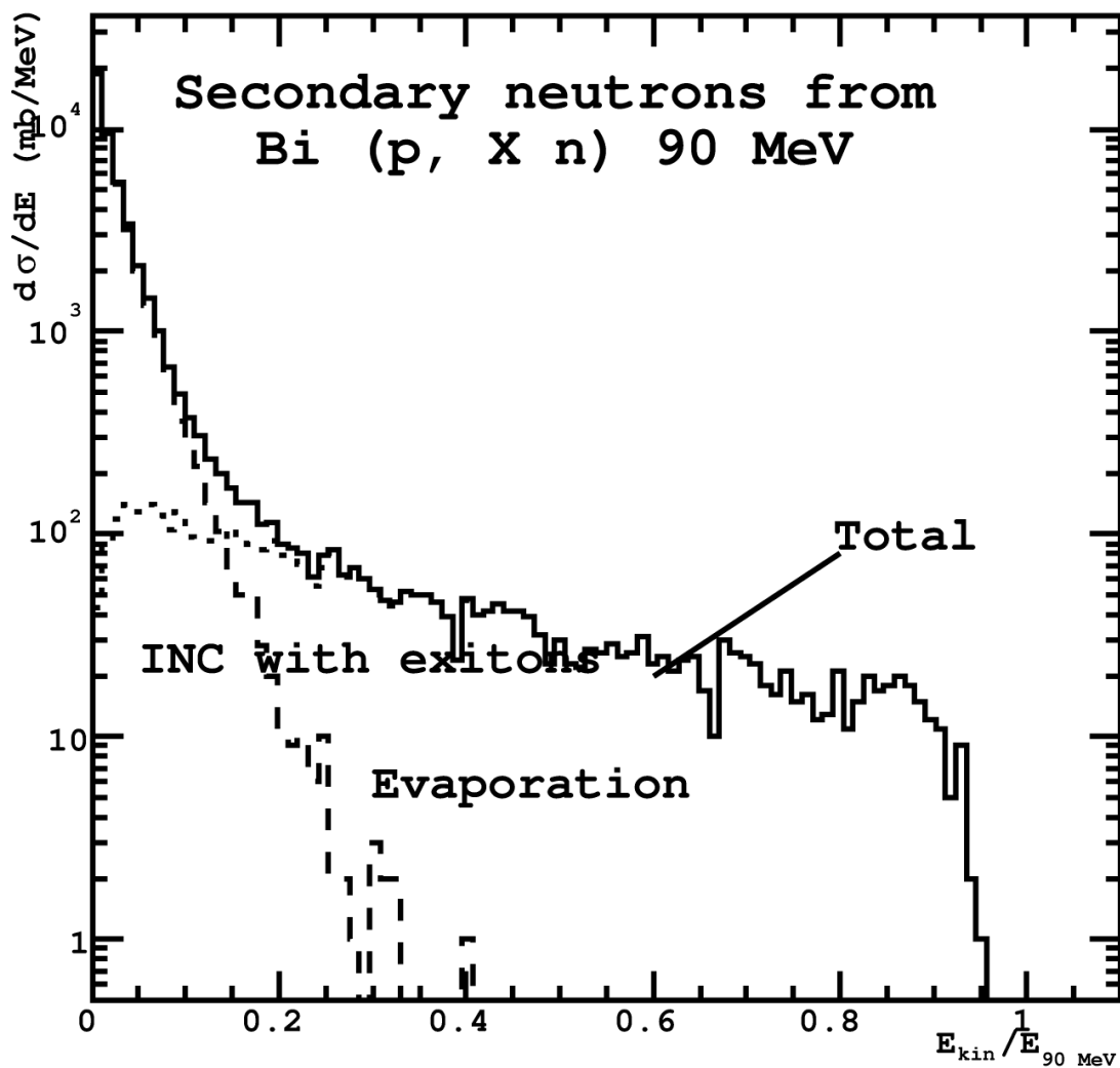
Fig. 26.1: Secondary neutrons generated by Bertini INC with excitons and evaporation model.
