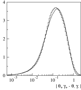
Fig. 6.15: Distribution of the difference of transverse momenta of positive and negative muons (with logarithmic x-scale).
