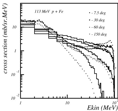
Fig. 27.5: Double differential cross-section for neutrons produced in proton scattering off Iron. Proton incident energy was 113 MeV. The points are data, the histogram is Binary Cascade prediction.
