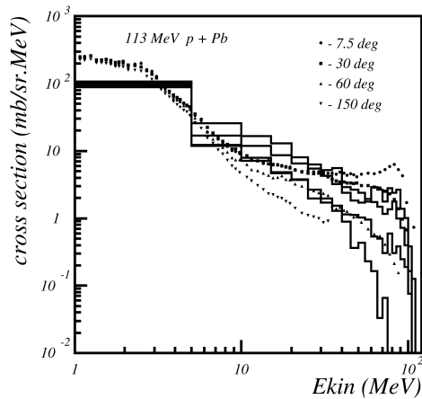
Fig. 27.9: Double differential cross-section for neutrons produced in proton scattering off Lead. Proton incident energy was 113 MeV. The points are data, the histogram is Binary Cascade prediction.
