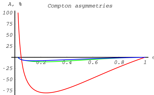
Fig. 13.21: Compton scattering differential cross section asymmetries in%. Red line corresponds to the asymmetry due to circular photon and longitudinal electron initial state polarization, green line – due to circular photon and transverse electron initial state polarization, blue line – due to linear photon and transverse electron initial state polarization.
