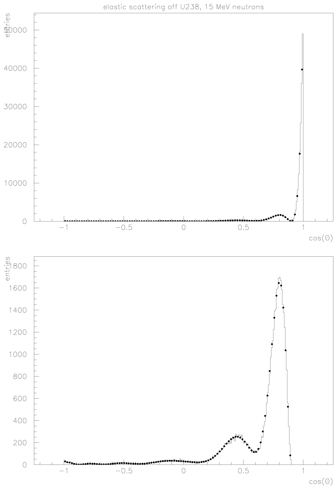
Fig. 39.1: Comparison of data and Monte Carlo for the angular distribution of 15 MeV neutrons scattered elastically off uranium ( ^{238}\text{U} ). The points are evaluated data, and the histogram is the Monte Carlo prediction. The lower plot excludes the forward peak, to better show the Frenel structure of the angular distribution of the scattered neutron.
