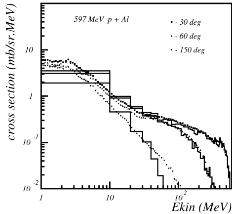
Fig. 27.3: Double differential cross-section for neutrons produced in proton scattering off Aluminum. Proton incident energy was 597 MeV. The points are data, the histogram is Binary Cascade prediction.
