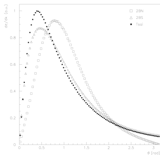
Fig. 10.3: Comparison of polar angle distribution of bremsstrahlung photons ( k/T = 0.5 ) for 100 keV electrons in silver, obtained with Tsai, 2BS and 2BN generator
