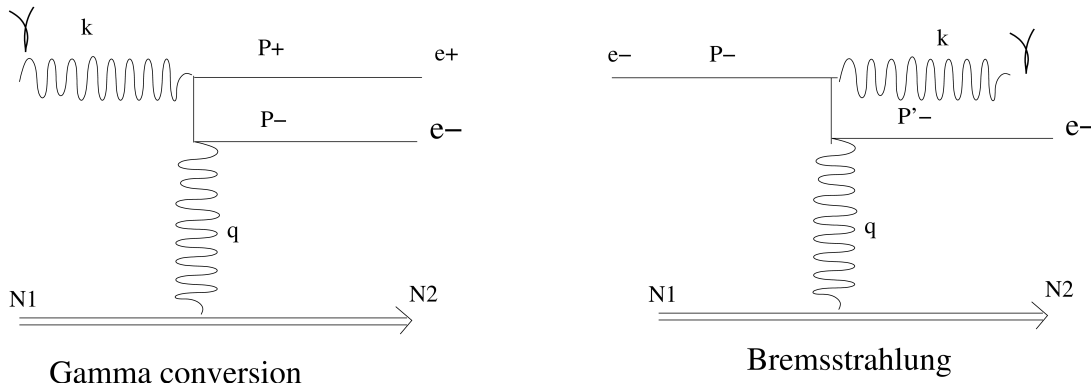
Fig. 13.24: Feynman diagrams of Gamma conversion and bremsstrahlung processes.
