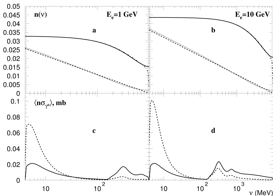
Fig. 44.1: Relative contribution of equivalent photons with small Q^2 to the total “photon flux” for (a) 1 GeV electrons and (b) 10 GeV electrons. In figures (c) and (d) the equivalent photon distribution dn(\nu, Q^2) is multiplied by the photonuclear cross section \sigma_{\gamma^*}(K, Q^2) and integrated over Q^2 in two regions: the dashed lines are integrals over the low- Q^2 equivalent photons (under the dashed line in the first two figures), and the solid lines are integrals over the high- Q^2 equivalent photons (above the dashed lines in the first two figures).
