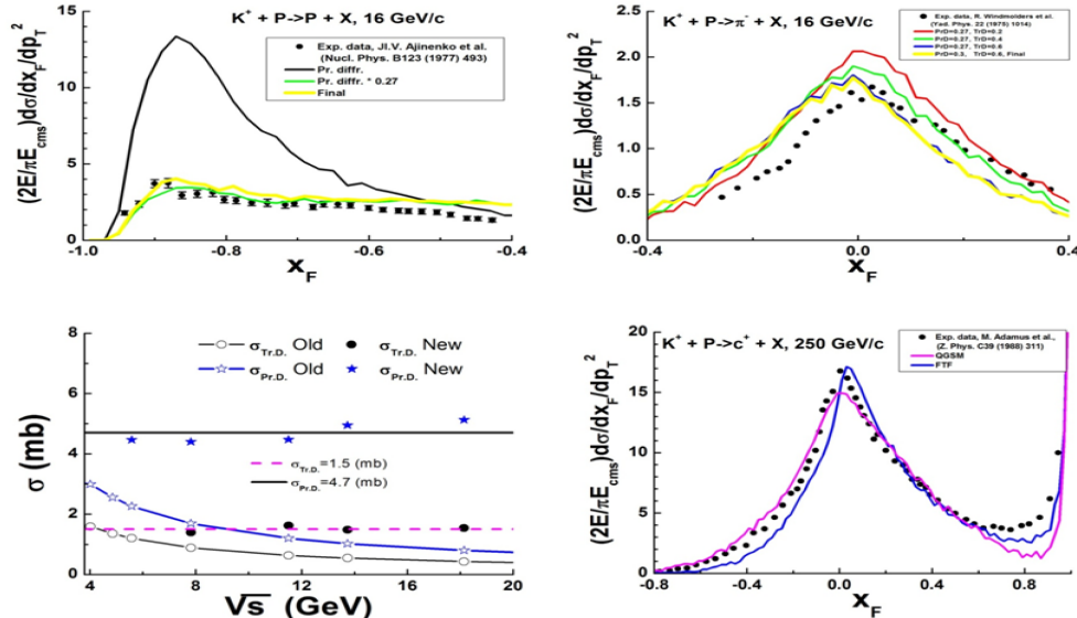
Fig. 25.13: Upper figures: inclusive spectra of protons and \pi^+ -mesons in Kp -interactions. Points are experimental data [eal86][eal77]. Lines are FTF calculations. Bottom left figure: diffraction dissociation cross sections obtained by tuning (points), and their description (lines) by the expression for Kp in (25.4). Bottom right figure: x_F spectrum of positive charged particles in Kp -interactions at p_{\text{lab}} = 250 GeV/c. Points are experimental data [Whi74], lines are model calculations.
