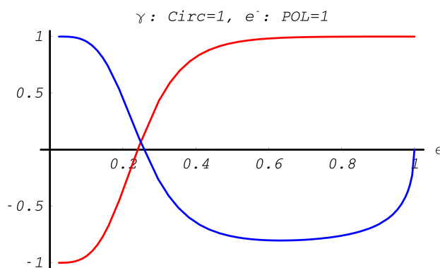
Fig. 13.22: Polarization Transfer in Compton scattering. Blue line corresponds to the longitudinal polarization \xi_3^{(2)} of the electron, red line – circular polarization \xi_3^{(1)} of the photon.
