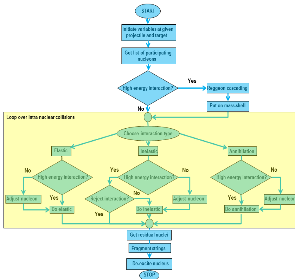
Fig. 25.14: Flowchart of the FTF model.
