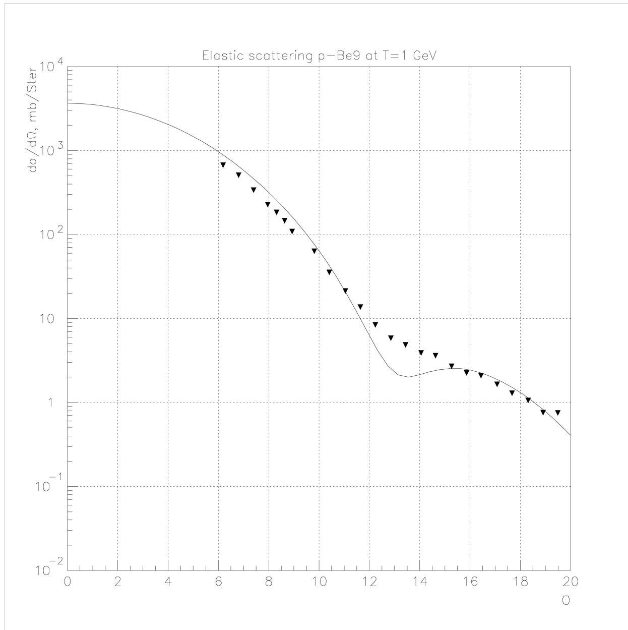
Fig. 23.1: Elastic proton scattering on ^9\text{Be} at 1 GeV.
