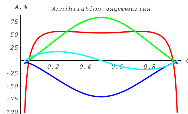
Fig. 13.15: Annihilation differential cross section asymmetries in %. Red line corresponds to A_{ZZ}(\epsilon) , green line – A_{XX}(\epsilon) , blue line – A_{YY}(\epsilon) , lightblue line – A_{ZX}(\epsilon) . Kinetic energy of the incoming positron T_{k_1} = 10\text{MeV} .
