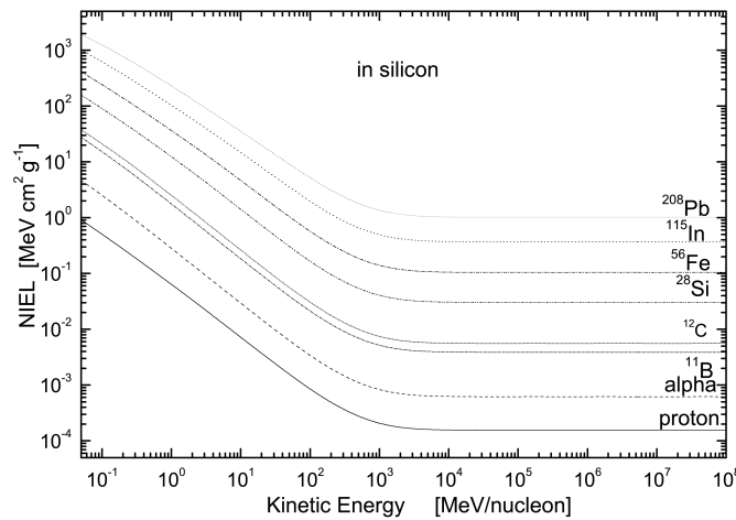
Fig. 8.3: Non-ionizing stopping power from Ref. [eal11] calculated using Eq.(8.33) in silicon is shown as a function of the kinetic energy per nucleon, from 50 keV/nucleon up 100 TeV/nucleon, for protons, \alpha -particles and ^{11}\text{B} , ^{12}\text{C} , ^{28}\text{Si} , ^{56}\text{Fe} , ^{115}\text{In} , ^{208}\text{Pb} nuclei. The threshold energy for displacement is 21 eV in silicon.
