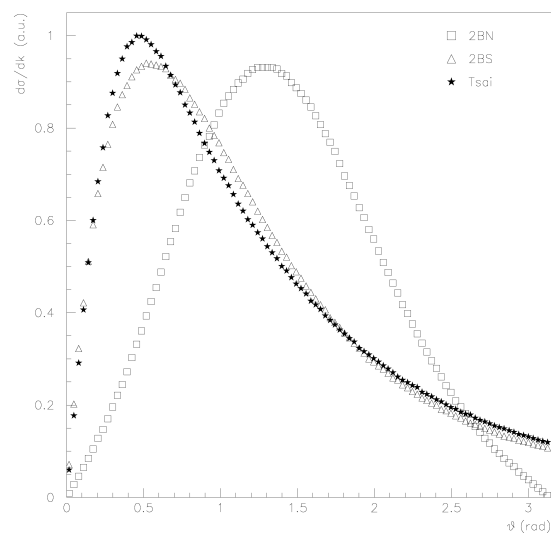
Fig. 10.2: Comparison of polar angle distribution of bremsstrahlung photons ( k/T = 0.5 ) for 10 keV electrons in silver, obtained with Tsai, 2BS and 2BN generator
