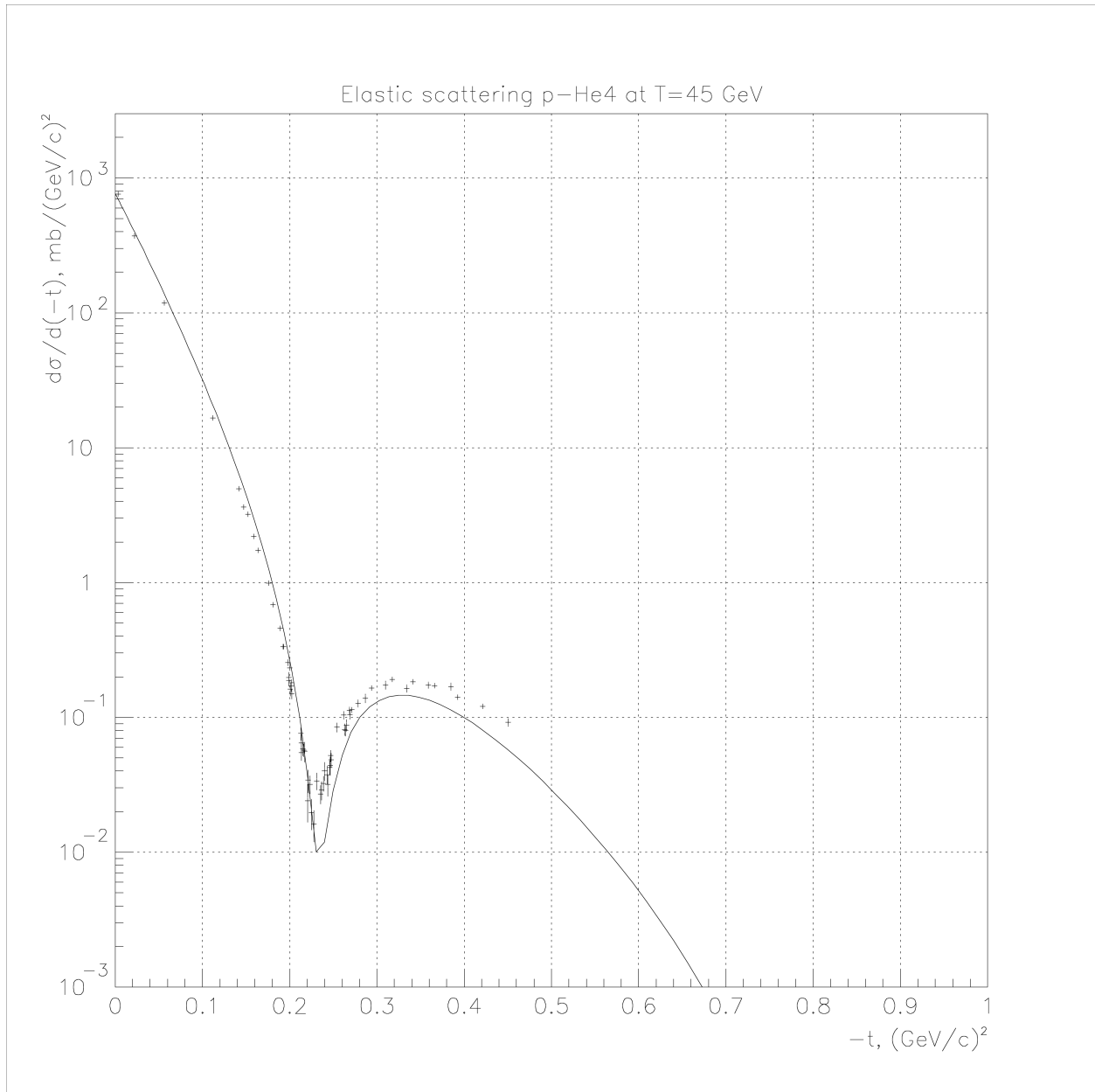
Fig. 23.11: Elastic proton scattering on ^4\text{He} at 45 GeV.
