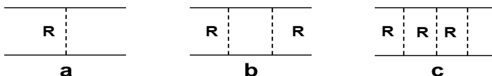
Fig. 25.16: Nonenhanced diagrams of NN -scattering.
