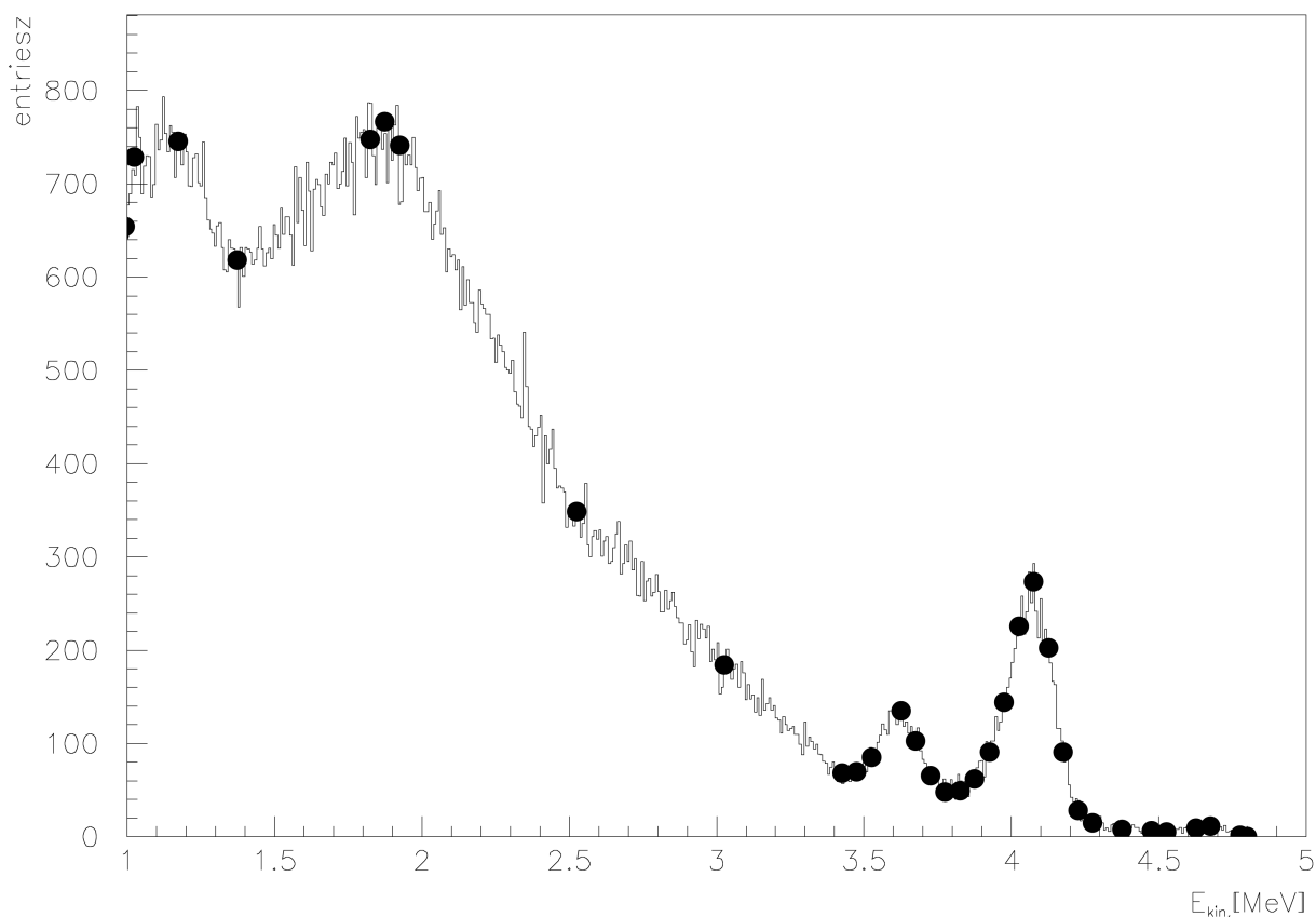
Fig. 39.2: Comparison of data and Monte Carlo for photon energy distributions for radiative capture of 15 MeV neutrons on Uranium ( ^{238}\text{U} ). The points are evaluated data, the histogram is the Monte Carlo prediction.
