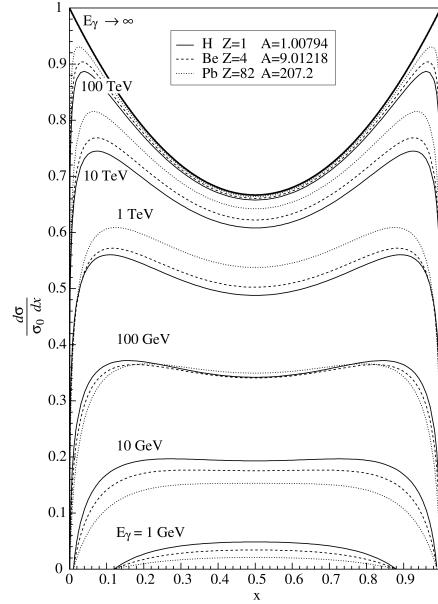
Fig. 6.3: Normalized differential cross section for pair production as a function of x , the energy fraction of the photon energy carried by one of the leptons in the pair. The function is shown for three different elements, hydrogen, beryllium and lead, and for a wide range of photon energies.
