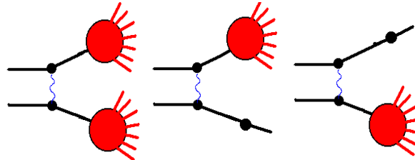
Fig. 25.1: Non-diffractive and diffractive interactions considered in the Fritiof model.
