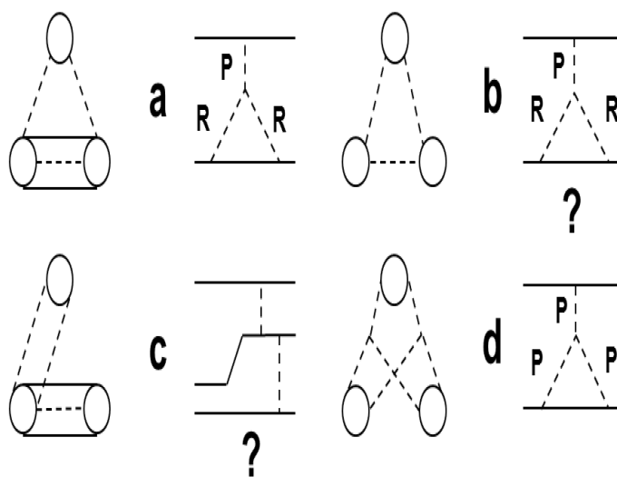
Fig. 25.21: Diagrams of quark-gluon exchanges and corresponding reggeon diagrams for hadron-nucleus interactions.
