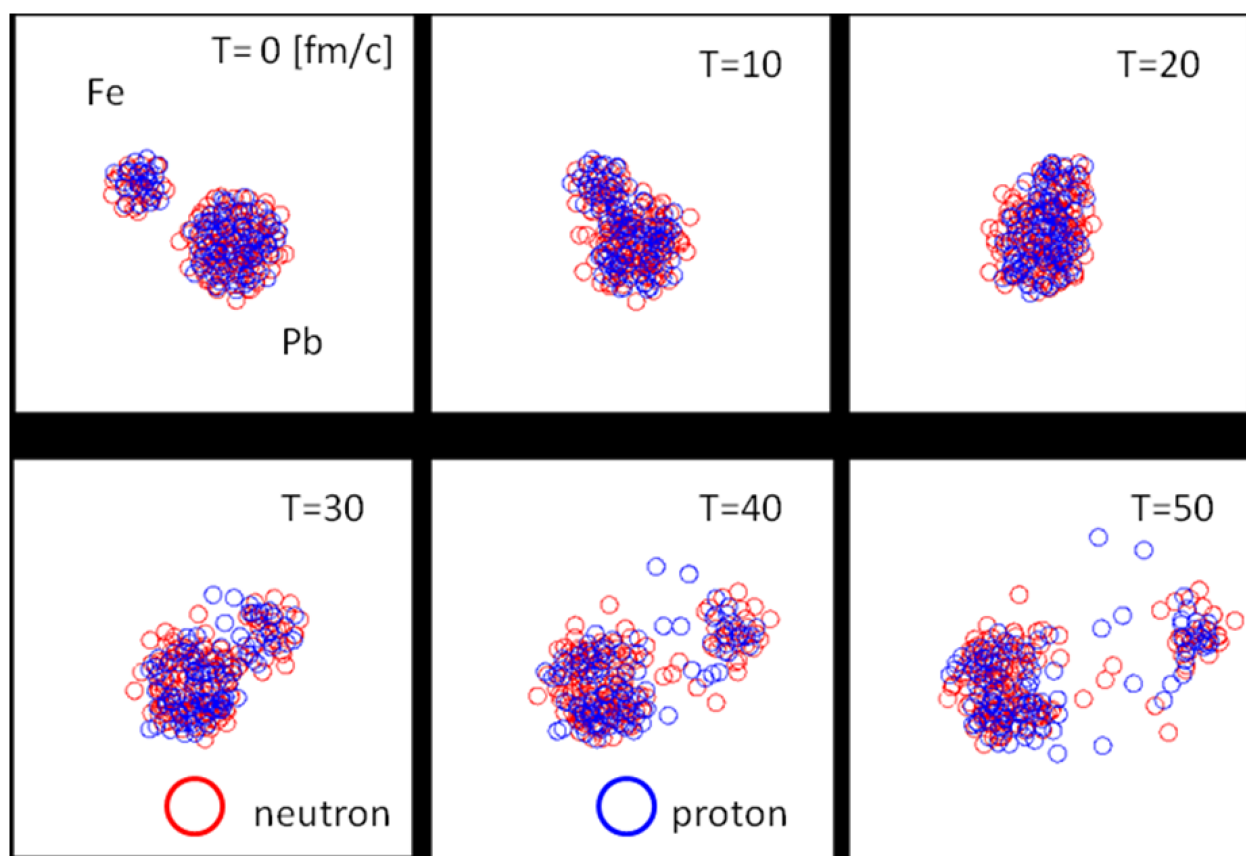
Fig. 35.1: Time evolution of reaction of 290 MeV/n Fe on Pb in position space. Red and Blue circle represents neutron and proton respectively. Full scale of each panel is 50 fm.
