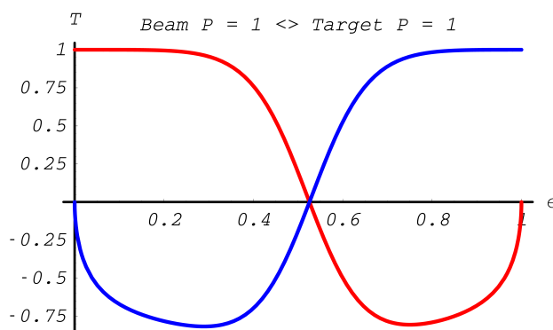
Fig. 13.10: Polarization Transfer in Bhabha scattering. Longitudinal polarization \xi_3^{(2)} of electron with energy E_{p_2} in blue; longitudinal polarization \xi_3^{(1)} of scattered positron. Kinetic energy of incoming positron T_{k_1} = 10\text{MeV}
