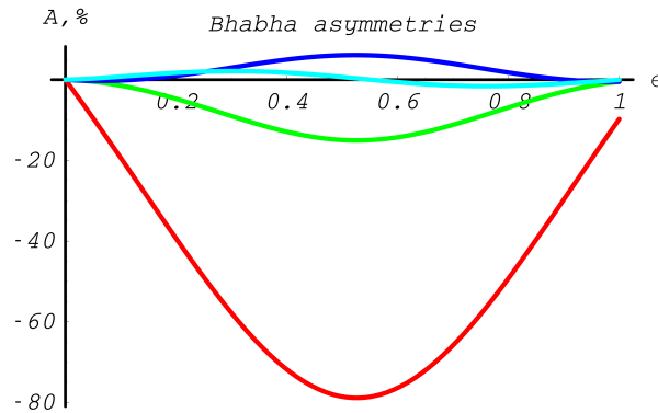
Fig. 13.7: Differential cross section asymmetries in % for Bhabha scattering (red - A_{ZZ}(\epsilon) , green - A_{XX}(\epsilon) , blue - A_{YY}(\epsilon) , light blue - A_{ZX}(\epsilon) )
