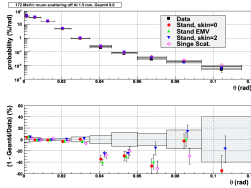
Fig. 8.1: Scattering of muons off 1.5 mm aluminum foil: data [eal06] - black squares; simulation - colored markers corresponding different options of multiple scattering and single scattering model; in the bottom plot - relative difference between the simulation and the data in percents; hashed area demonstrates one standard deviation of the data.
