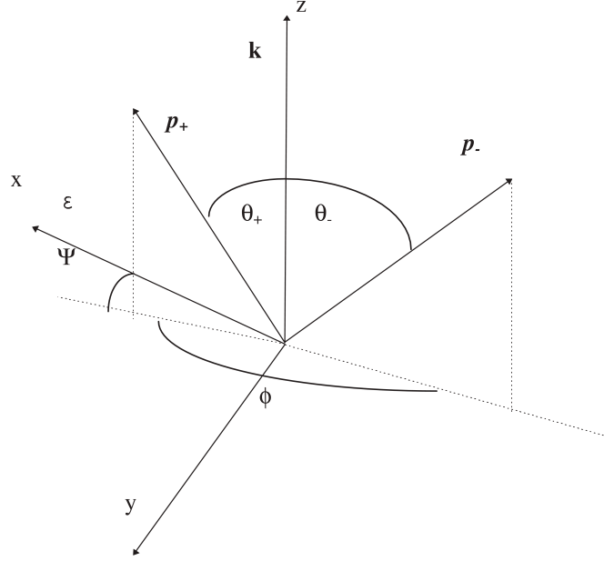
Fig. 13.25: Angles occurring in the pair creation
