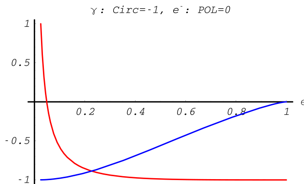
Fig. 13.23: Polarization Transfer in Compton scattering. Blue line corresponds to the longitudinal polarization \xi_3^{(2)} of the electron, red line – circular polarization \xi_3^{(1)} of the photon.
