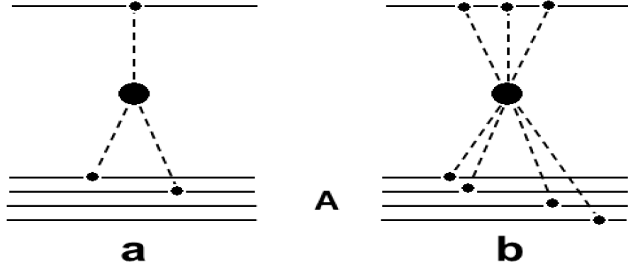
Fig. 25.18: Possible enhanced diagrams of hA -interactions.
