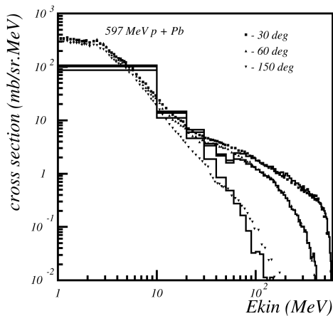
Fig. 27.11: Double differential cross-section for neutrons produced in proton scattering off Lead. Proton incident energy was 597 MeV. The points are data, the histogram is Binary Cascade prediction.
