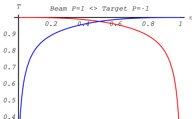
Fig. 13.9: Polarization transfer functions in Møller scattering. Longitudinal polarization \xi_3^{(2)} of electron with energy E_{p_2} in blue; longitudinal polarization \xi_3^{(1)} of second electron in red. Kinetic energy of incoming electron T_{k_1} = 10\text{MeV}
