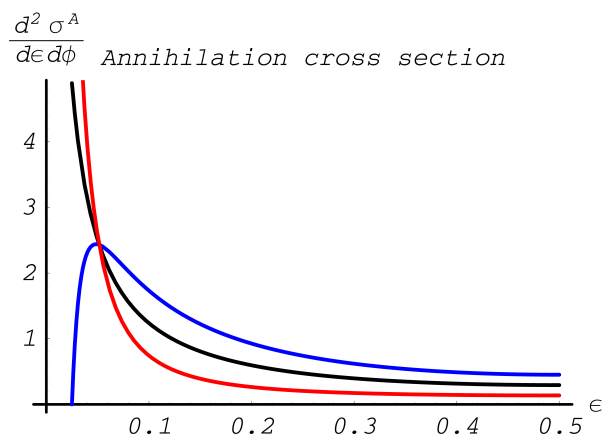
Fig. 13.14: Annihilation differential cross section in arbitrary units. Black line corresponds to unpolarized cross section; red line – to the antiparallel spins of initial particles, and blue line – to the parallel spins. Kinetic energy of the incoming positron T_{k_1} = 10\text{MeV} .
