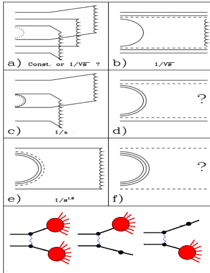
Fig. 25.10: Quark flow diagrams of \bar{p}p -interactions.
