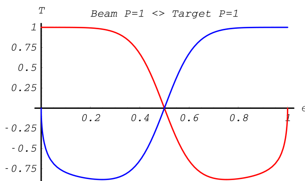
Fig. 13.8: Polarization transfer functions in Møller scattering. Longitudinal polarization \xi_3^{(2)} of electron with energy E_{p_2} in blue; longitudinal polarization \xi_3^{(1)} of second electron in red. Kinetic energy of incoming electron T_{k_1} = 10\text{MeV}
