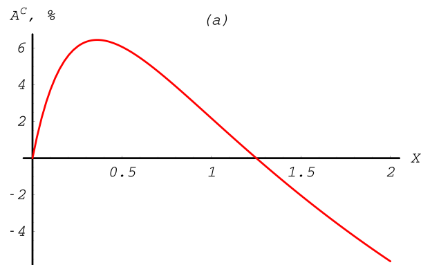
Fig. 13.18: Compton total cross section asymmetry depending on the energy of incoming photon. Between 0 and \sim 1 MeV.
