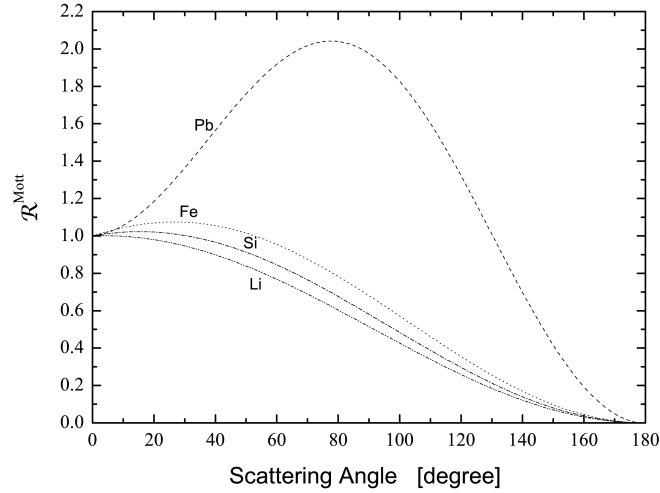
Fig. 8.4: \mathcal{R}^{\text{Mott}} obtained from Eq.(8.48) at 100 MeV for Li, Si, Fe and Pb nuclei as a function of scattering angle.
