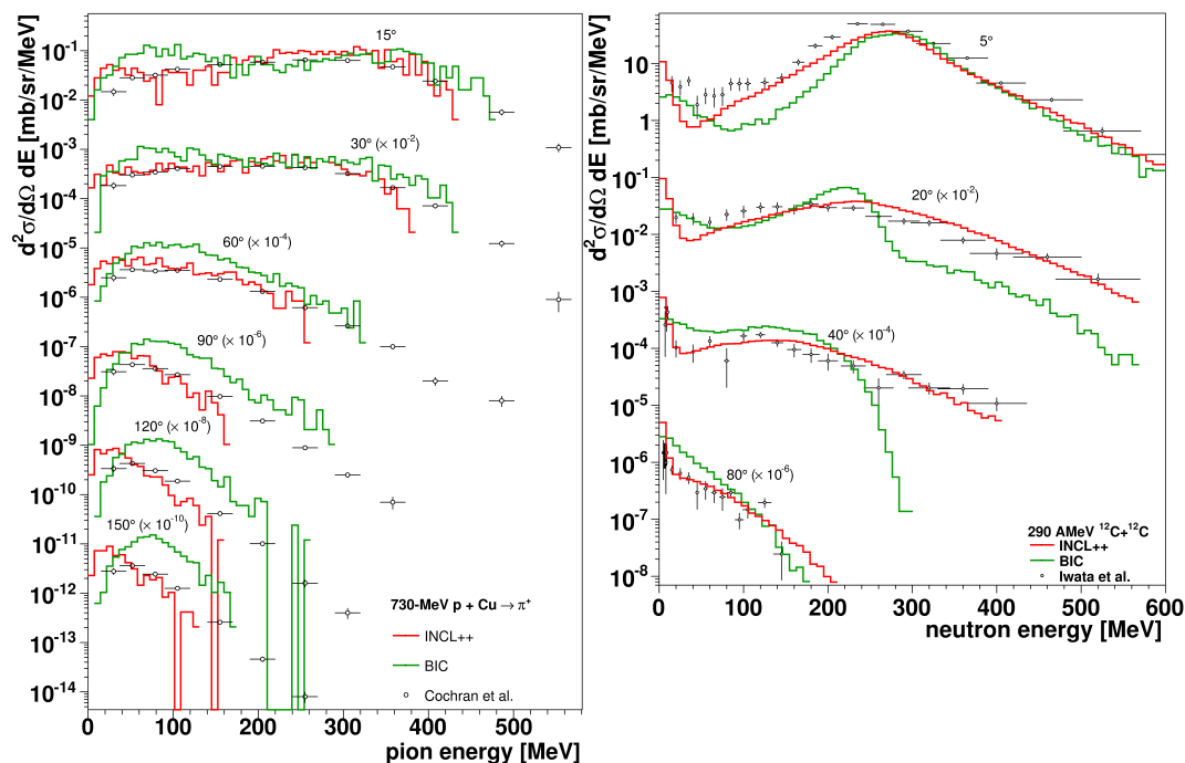
Fig. 28.2: Left: double-differential cross sections for the production of charged pions in 730-MeV p+\text{Cu} . Right: double-differential cross sections for the production of neutrons in 290-AMeV ^{12}\text{C}+^{12}\text{C} . Predictions of the INCL++ and Binary-Cascade models are compared with experimental data from Refs. [CDG+72] and [IMS+01].
