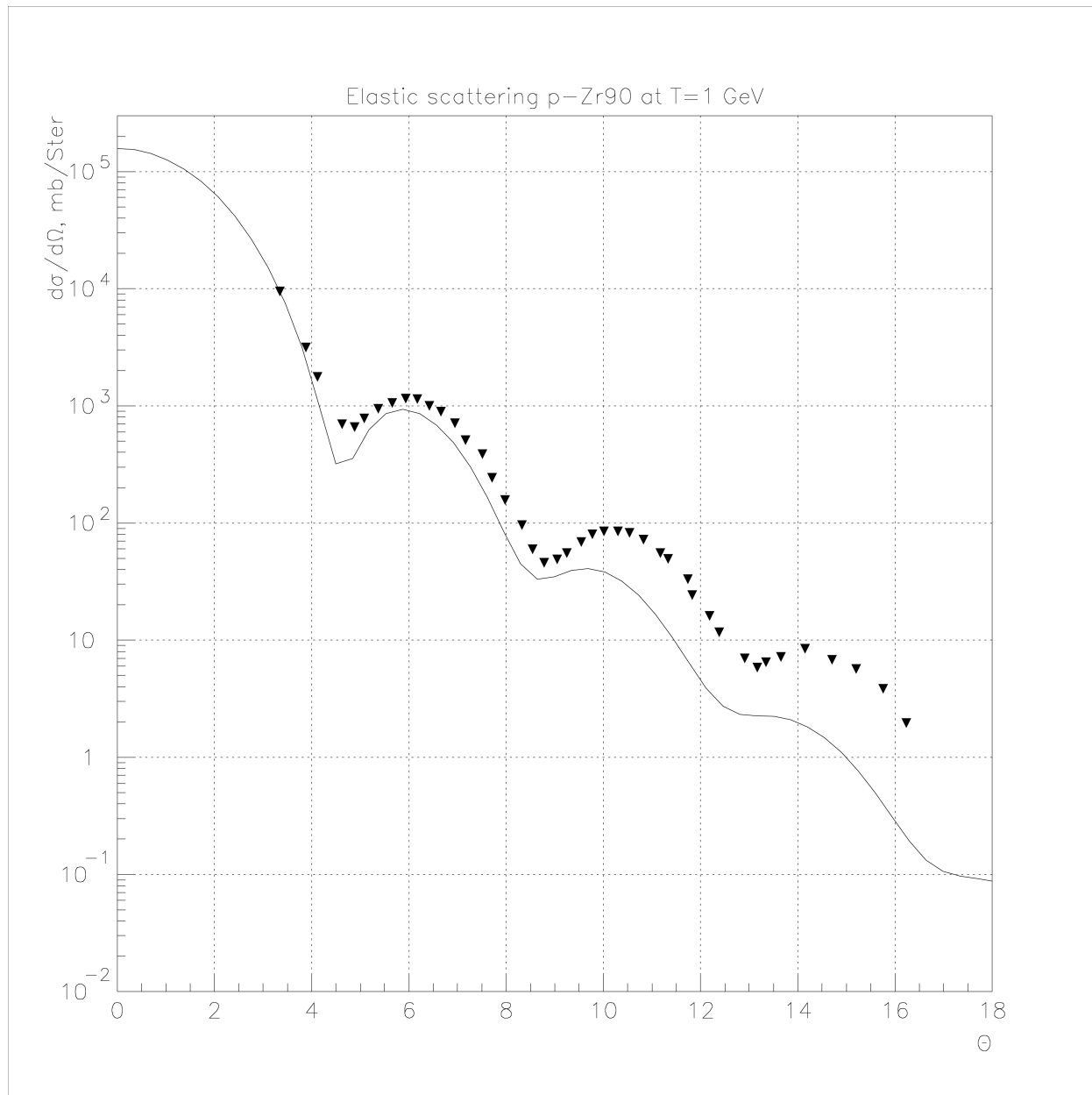
Fig. 23.8: Elastic proton scattering on ^{90}\text{Zr} at 1 GeV.
