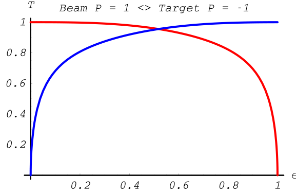
Fig. 13.11: Polarization Transfer in Bhabha scattering. Longitudinal polarization \xi_3^{(2)} of electron with energy E_{p_2} in blue; longitudinal polarization \xi_3^{(1)} of scattered positron. Kinetic energy of incoming positron T_{k_1} = 10\text{MeV}
