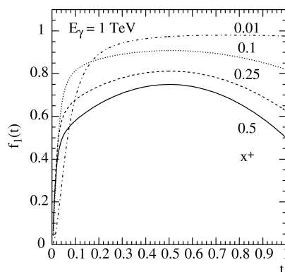
Fig. 6.8: The function f_1(t) at E_\gamma = 1 TeV in beryllium for different values of x_+ .
