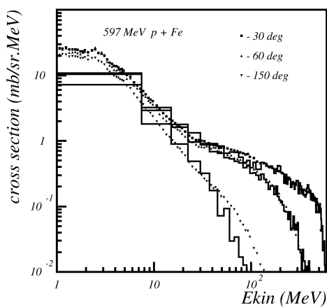
Fig. 27.7: Double differential cross-section for neutrons produced in proton scattering off Iron. Proton incident energy was 597 MeV. The points are data, the histogram is Binary Cascade prediction.
