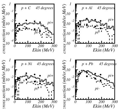
Fig. 27.13: Double differential cross-section for pions produced at 45^\circ in proton scattering off various materials. Proton incident energy was 597 MeV in each case. The points are data, the histogram is Binary Cascade prediction.
