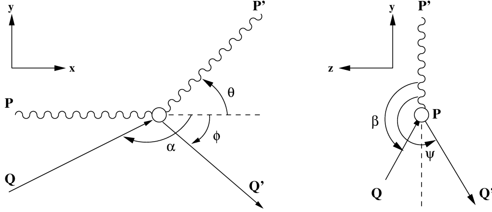
Fig. 6.1: Scattering diagram of atomic bound electron Compton scattering. \mathbf{P} is the incident photon momentum, \mathbf{Q} the electron pre-collision momentum, \mathbf{P}' the scattered photon momentum and \mathbf{Q}' the recoil electron momentum.
