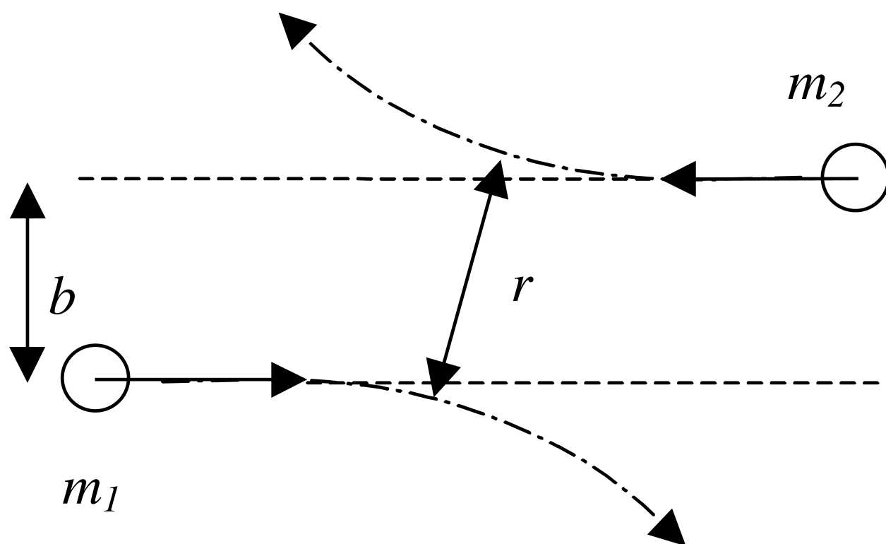
Fig. 36.2: Illustration clarifying impact parameter in the far-field ( b ) and actual impact parameter ( r ).
