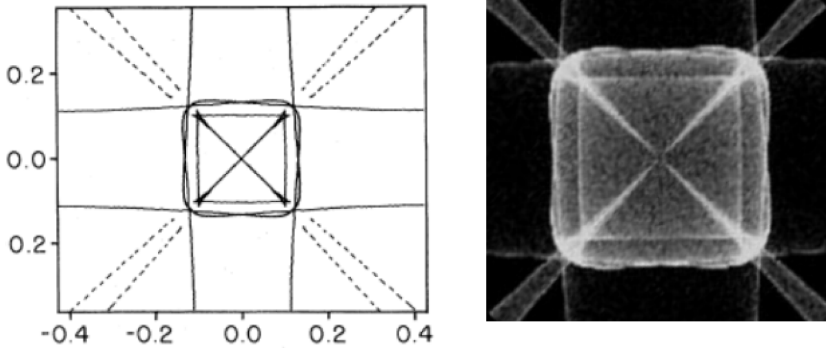
Fig. 19.1: Left: outline of phonon caustics in germanium as predicted by Northrop and Wolfe [NW79]. Right: Phonon caustics as simulated using the GEANT4 phonon transport code.
