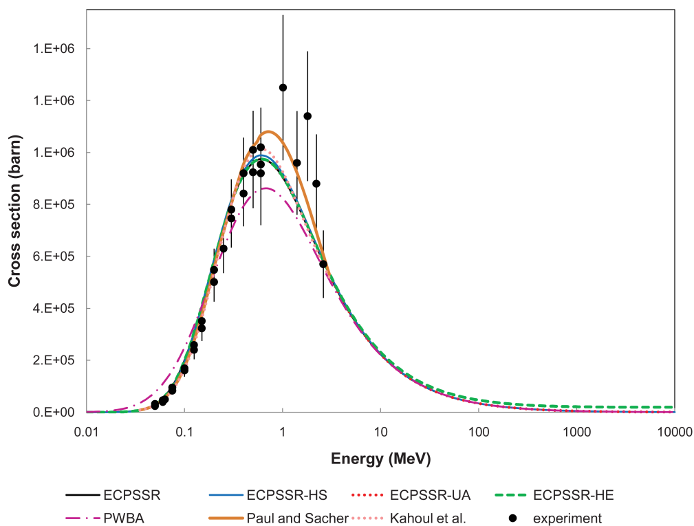
Fig. 9.2: Cross section for the ionisation of carbon K shell by proton impact according to the various implemented modeling options, and comparison with experimental data [PS89]: ECPSSR model, ECPSSR model with “united atom” (UA) approximation, Hartree-Slater (HS) corrections and specialized for high energies (HE); plane wave Born approximation (PWBA); empirical models by Paul and Sacher and Kahoul et al. The curves reproducing some of the model implementations can be hardly distinguished in the plot due to their similarity.
