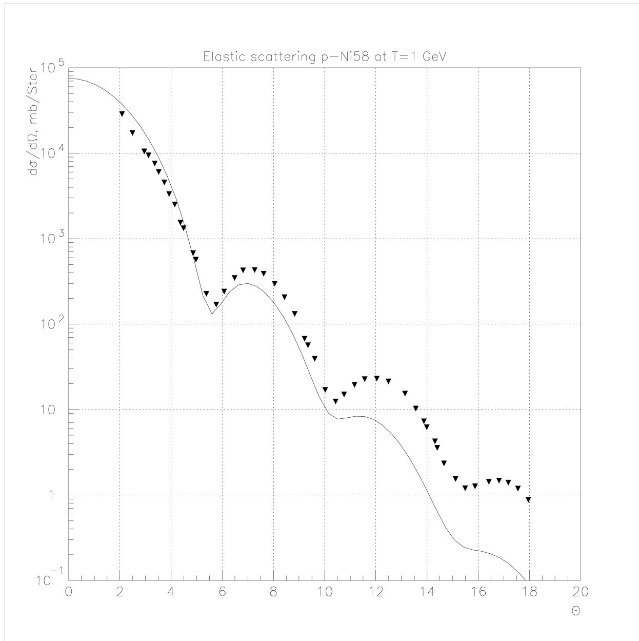
Fig. 23.7: Elastic proton scattering on ^{58}\text{Ni} at 1 GeV.
