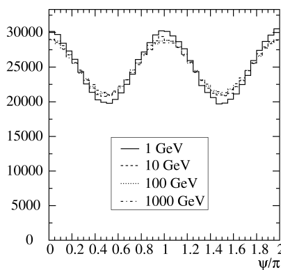
Fig. 6.10: Histograms of generated \psi distributions for beryllium at four different photon energies.
