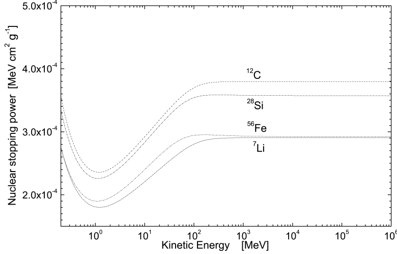
Fig. 8.5: In \text{MeVcm}^2/\text{g} , nuclear stopping powers in {}^7\text{Li} , {}^{12}\text{C} , {}^{28}\text{Si} and {}^{56}\text{Fe} calculated from Eq.(8.75) and divided by the density of the material as a function of the kinetic energy of electrons from 200 keV up to 1 TeV.
