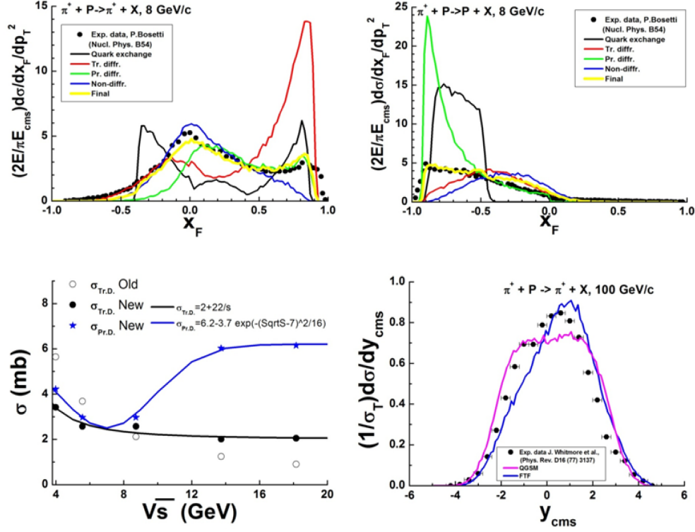
Fig. 25.12: Upper figures: inclusive spectra of protons and \pi^+ -mesons in \pi^+p -interactions. Points are experimental data [eal73b]. Lines represent the contributions of the various FTF processes calculated by assuming that the probability of each process is 100 %. Bottom left figure: diffraction dissociation cross sections obtained by tuning (points), and their description (lines) by the expression for \pi in (25.4). Bottom right figure: rapidity spectrum of \pi^+ -mesons in \pi^+p -interactions at p_{\text{lab}} = 100 GeV/c. Points are experimental data [Whi74].
