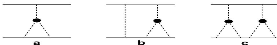
Fig. 25.17: Simplest enhanced diagrams of NN -scattering.
