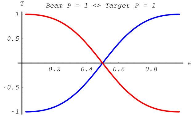
Fig. 13.16: Polarization Transfer in annihilation process. Blue line corresponds to the circular polarization \xi_3^{(1)} of the photon with energy m(\gamma + 1)\epsilon ; red line – circular polarization \xi_3^{(2)} of the photon with energy m(\gamma + 1)(1 - \epsilon) .
