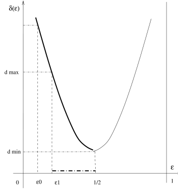
Fig. 6.2: Calculation of \epsilon for gamma conversion.
