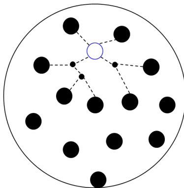
Fig. 25.19: Reggeon "cascade" in hA-scattering.
