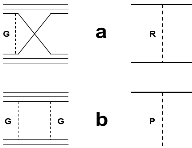
Fig. 25.20: Diagrams of quark-gluon exchanges and corresponding reggeon diagrams for hadron-nucleus interactions.
