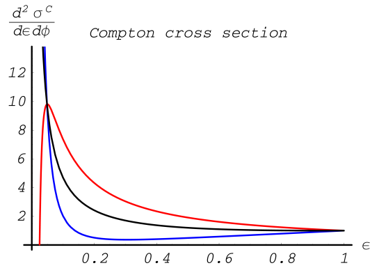
Fig. 13.20: Compton scattering differential cross section in arbitrary units. Black line corresponds to the unpolarized cross section; red line – to the antiparallel spins of initial particles, and blue line – to the parallel spins. Energy of the incoming photon E_{k_1} = 10\text{MeV} .
