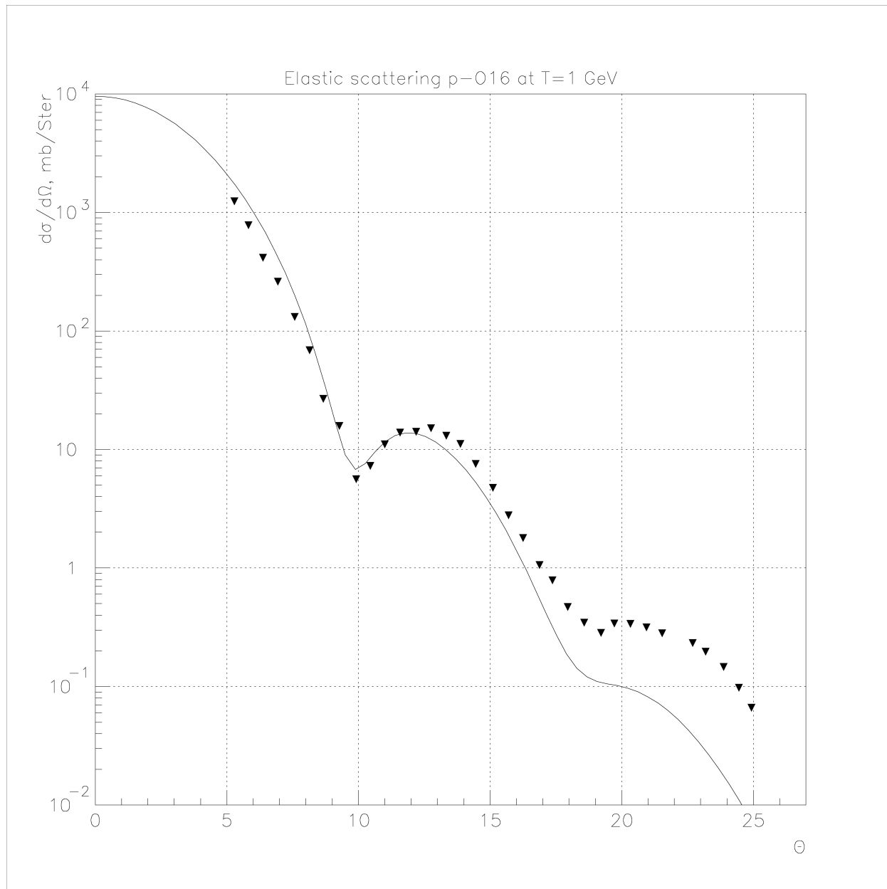
Fig. 23.4: Elastic proton scattering on 16 O at 1 GeV.
