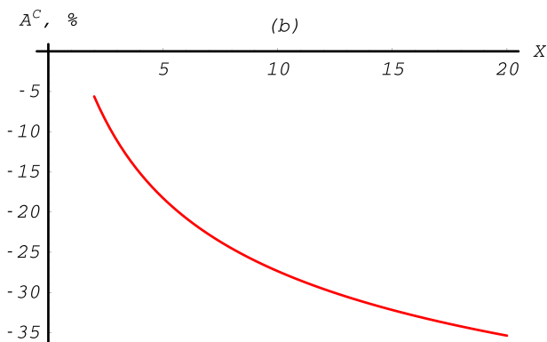
Fig. 13.19: Compton total cross section asymmetry depending on the energy of incoming photon. Up to 10MeV.
