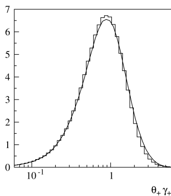
Fig. 6.14: Angular distribution in logarithmic scale. The curve corresponds to the exact calculations and the histogram is the simulated distribution.
