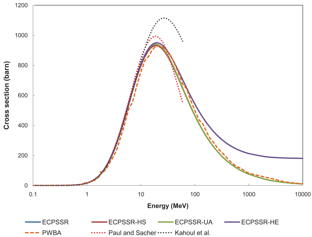
Fig. 9.1: Cross section for the ionisation of copper K shell by proton impact according to the various implemented modeling options: ECPSSR model, ECPSSR model with “united atom” (UA) approximation, Hartree-Slater (HS) corrections and specialized for high energies (HE); plane wave Born approximation (PWBA); empirical models by Paul and Sacher and Kahoul et al. The curves reproducing some of the model implementations can be hardly distinguished in the plot due to their similarity.
