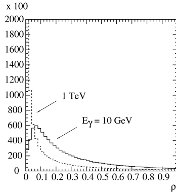
Fig. 6.11: Histograms of generated \rho distributions for beryllium at two different photon energies. The total number of entries at each energy is 10^6 .
