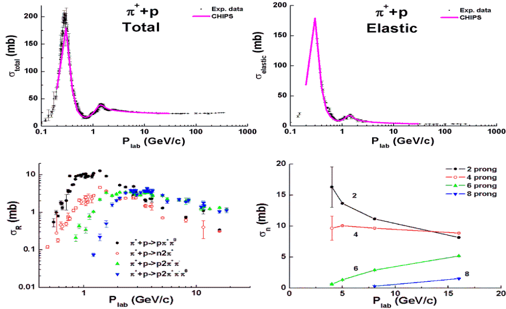
Fig. 25.5: General properties of \pi^+p -interactions. Points are experimental data: data on total and elastic cross sections from PDG data-base [PDG12], other data from [eal72].
