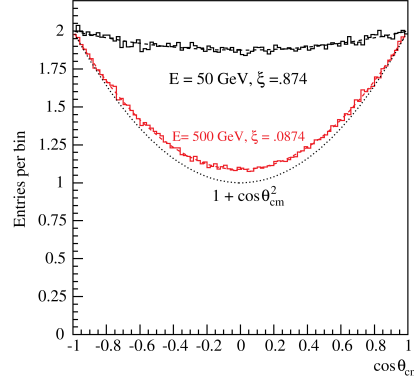
Fig. 10.7: Generated histograms with 10^6 entries each and the expected \cos \theta_{\text{cm}} distributions (dashed lines) at E = 50 and 500 GeV positron energy in the lab frame. The asymptotic 1 + \cos^2 \theta_{\text{cm}} distribution valid for E \rightarrow \infty is shown as dotted line.
