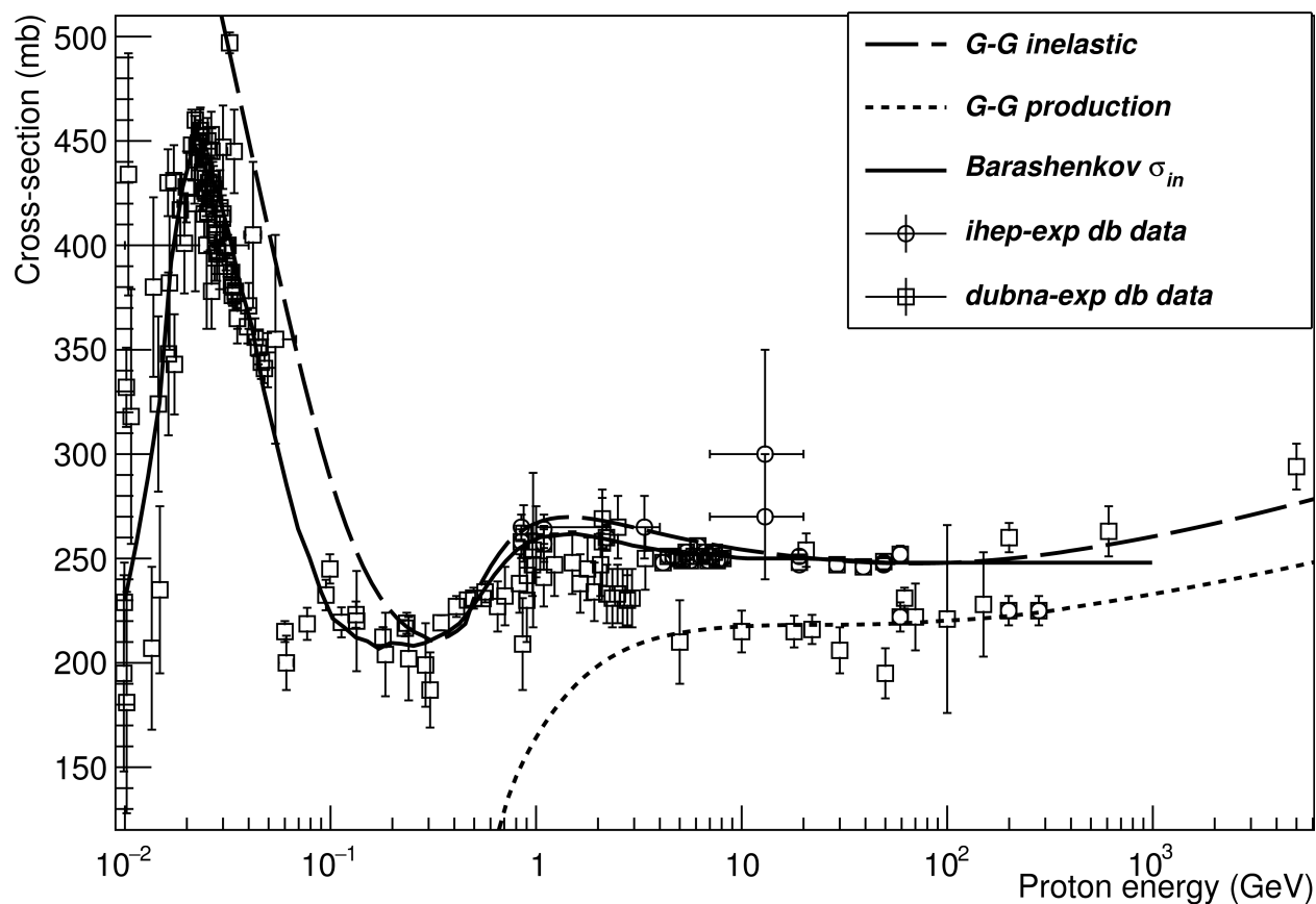
Fig. 21.2: Inelastic and production cross-sections of protons on a carbon target in the energy range 10^{-2} - 10^3 GeV. Experimental data (open points and squares) are from [IHEP][NEA]. The solid and dashed lines correspond to the Barashnikov and Glauber-Gribov inelastic models, respectively. The dotted line shows the Glauber-Gribov production model.
