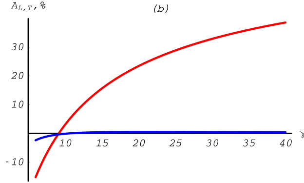
Fig. 13.13: Annihilation total cross section asymmetries depending on the total energy of the incoming positron E_{k_1} . The transverse asymmetry is shown in blue, the longitudinal asymmetry in red.
