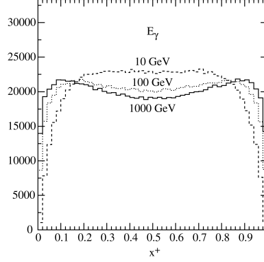
Fig. 6.6: Histogram of generated x_+ distributions for beryllium at three different photon energies. The total number of entries at each energy is 10^6 .
