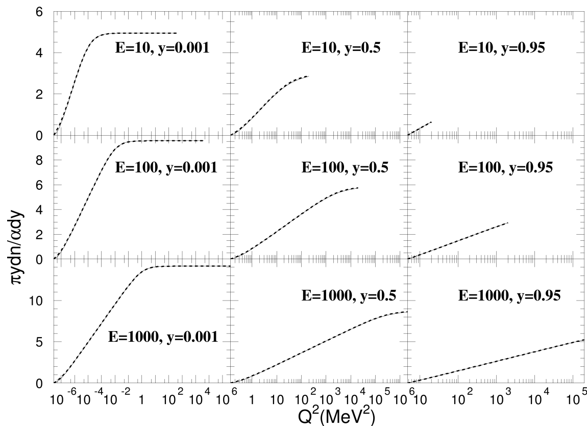
Fig. 44.2: Integrals of Q^2 spectra of virtual photons for three energies 10 MeV, 100 MeV, and 1 GeV at y=0.001 , y=0.5 , and y=0.95 . The solid line corresponds to Eq. (44.3) and the dashed line (which almost everywhere coincides with the solid line) corresponds to Eq. (44.8).
