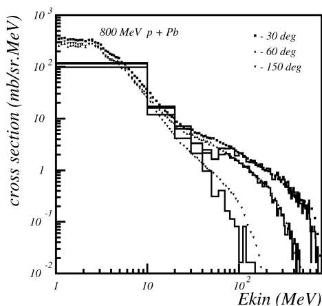
Fig. 27.12: Double differential cross-section for neutrons produced in proton scattering off Lead. Proton incident energy was 800 MeV. The points are data, the histogram is Binary Cascade prediction.
