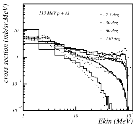
Fig. 27.1: Double differential cross-section for neutrons produced in proton scattering off Aluminum. Proton incident energy was 113 MeV.
