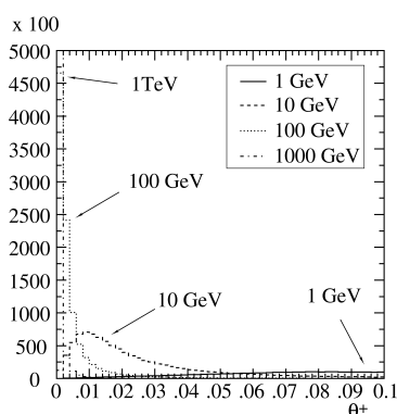
Fig. 6.12: Histograms of generated \theta_+ distributions at different photon energies.
