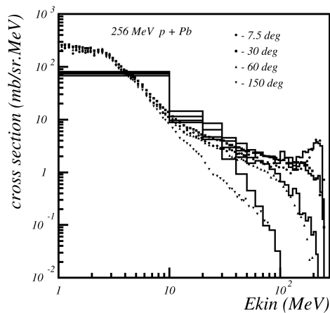
Fig. 27.10: Double differential cross-section for neutrons produced in proton scattering off Lead. Proton incident energy was 256 MeV. The points are data, the histogram is Binary Cascade prediction.
