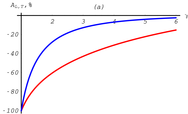
Fig. 13.12: Annihilation total cross section asymmetries depending on the total energy of the incoming positron E_{k_1} . The transverse asymmetry is shown in blue, the longitudinal asymmetry in red.
