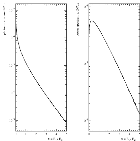
Fig. 14.3: Comparison of the exact (smooth curve) and generated (histogram) spectra for 2 \times 10^7 events. The photon spectrum is shown on the left and the power spectrum on the right side.
