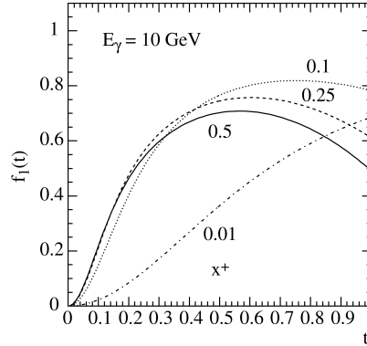
Fig. 6.7: The function f_1(t) at E_\gamma = 10 GeV in beryllium for different values of x_+ .
